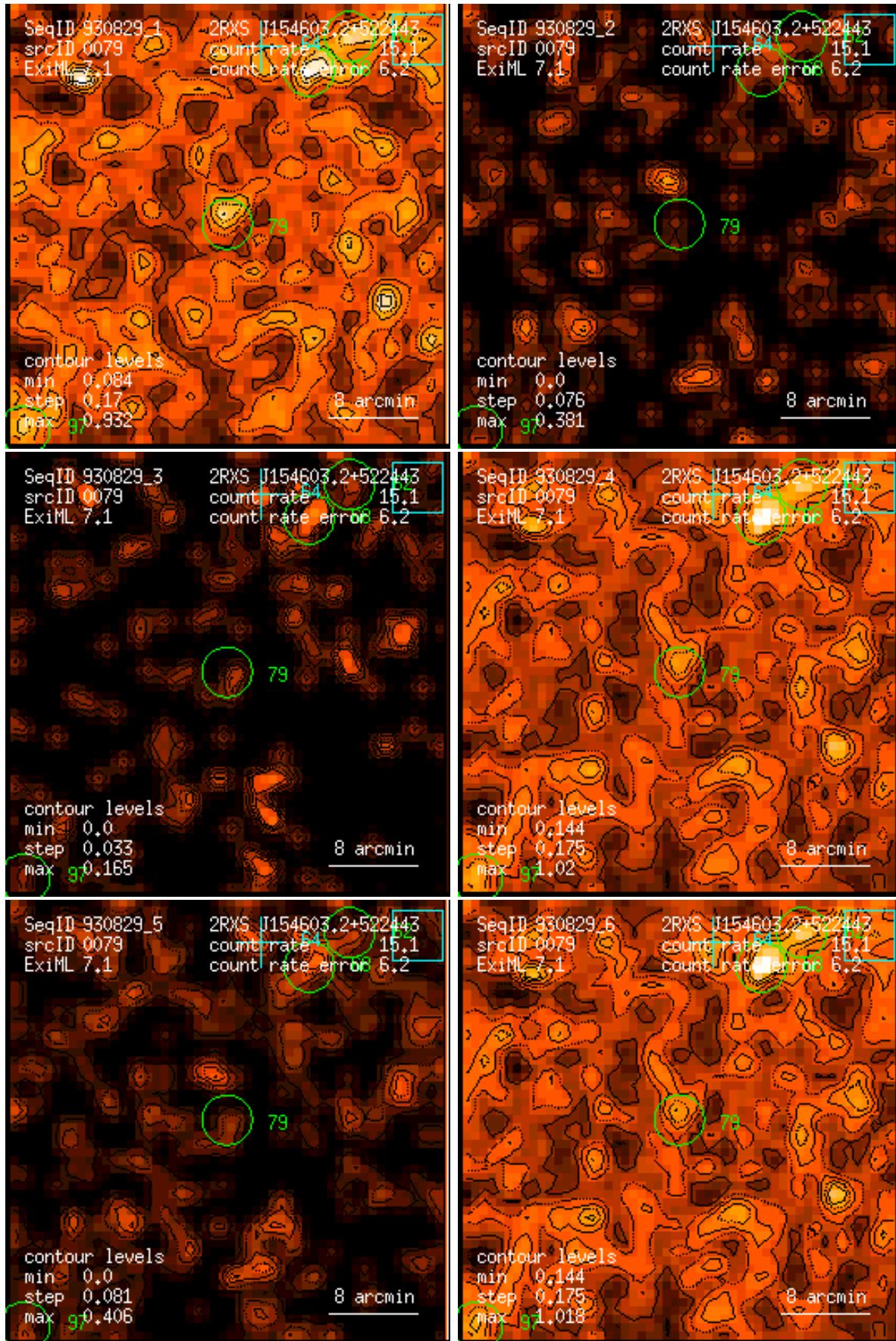
Figure 79: RASS 930829: detection 0079: band rate images, Gaussian filter: (1) PSPC channels 11 – 41, (2) 52 – 90, (3) 91 – 201, (4) 11 – 235, (5) 52 – 201, (6) 11 – 201. Broad band rates in counts/ks. Band rate contour levels in counts/ks/arcmin 2 .
