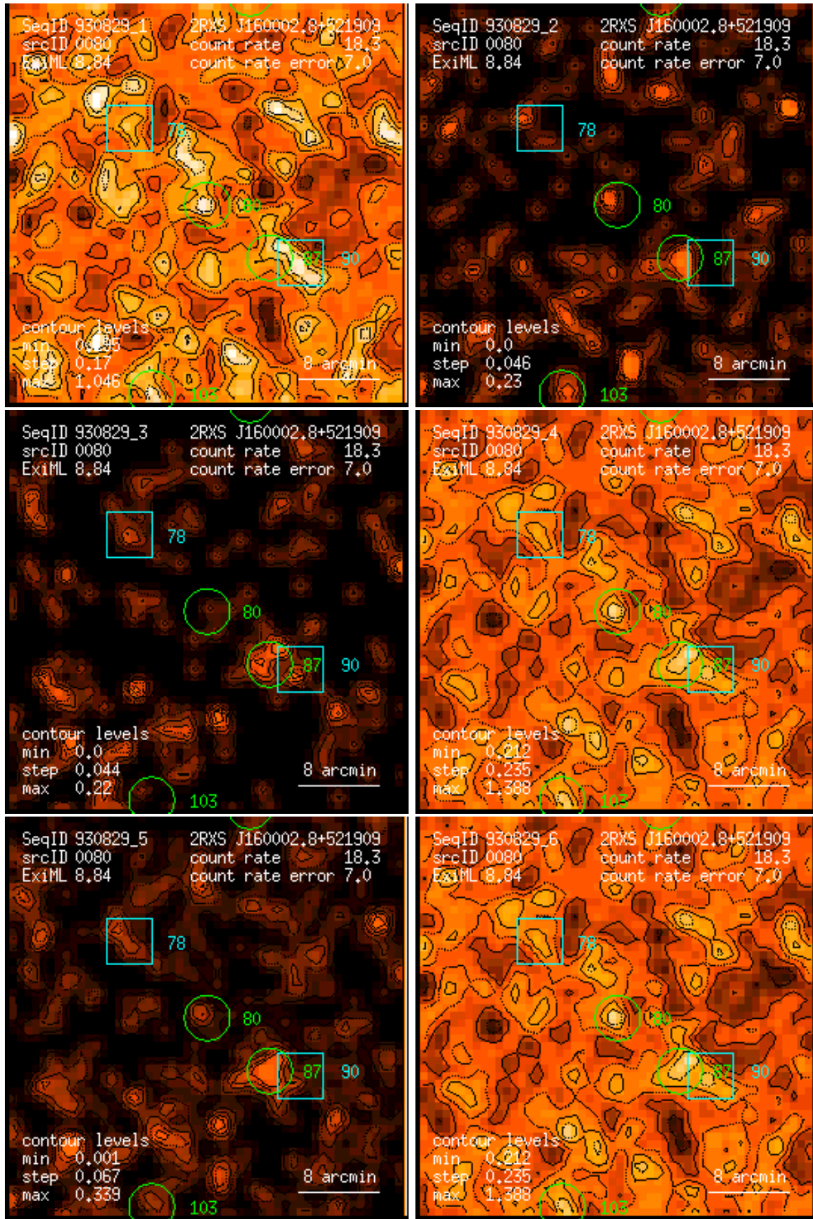
Figure 80: RASS 930829: detection 0080: band rate images, Gaussian filter: (1) PSPC channels 11 – 41, (2) 52 – 90, (3) 91 – 201, (4) 11 – 235, (5) 52 – 201, (6) 11 – 201. Broad band rates in counts/ks. Band rate contour levels in counts/ks/arcmin 2 .
