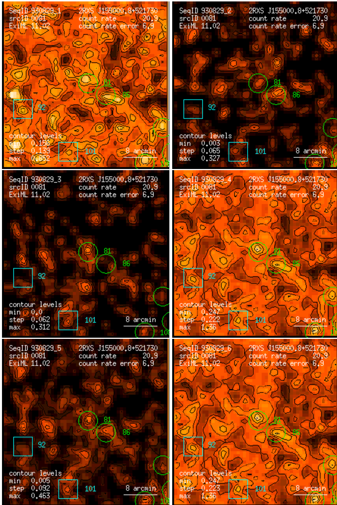
Figure 81: RASS 930829: detection 0081: band rate images, Gaussian filter: (1) PSPC channels 11 – 41, (2) 52 – 90, (3) 91 – 201, (4) 11 – 235, (5) 52 – 201, (6) 11 – 201. Broad band rates in counts/ks. Band rate contour levels in counts/ks/arcmin 2 .
