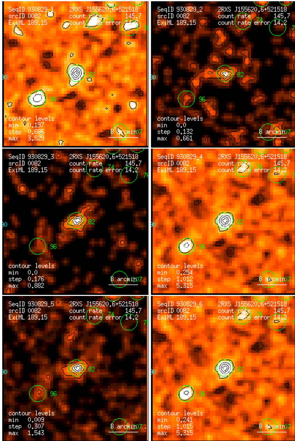
Figure 82: RASS 930829: detection 0082: band rate images, Gaussian filter: (1) PSPC channels 11 – 41, (2) 52 – 90, (3) 91 – 201, (4) 11 – 235, (5) 52 – 201, (6) 11 – 201. Broad band rates in counts/ks. Band rate contour levels in counts/ks/arcmin 2 .
