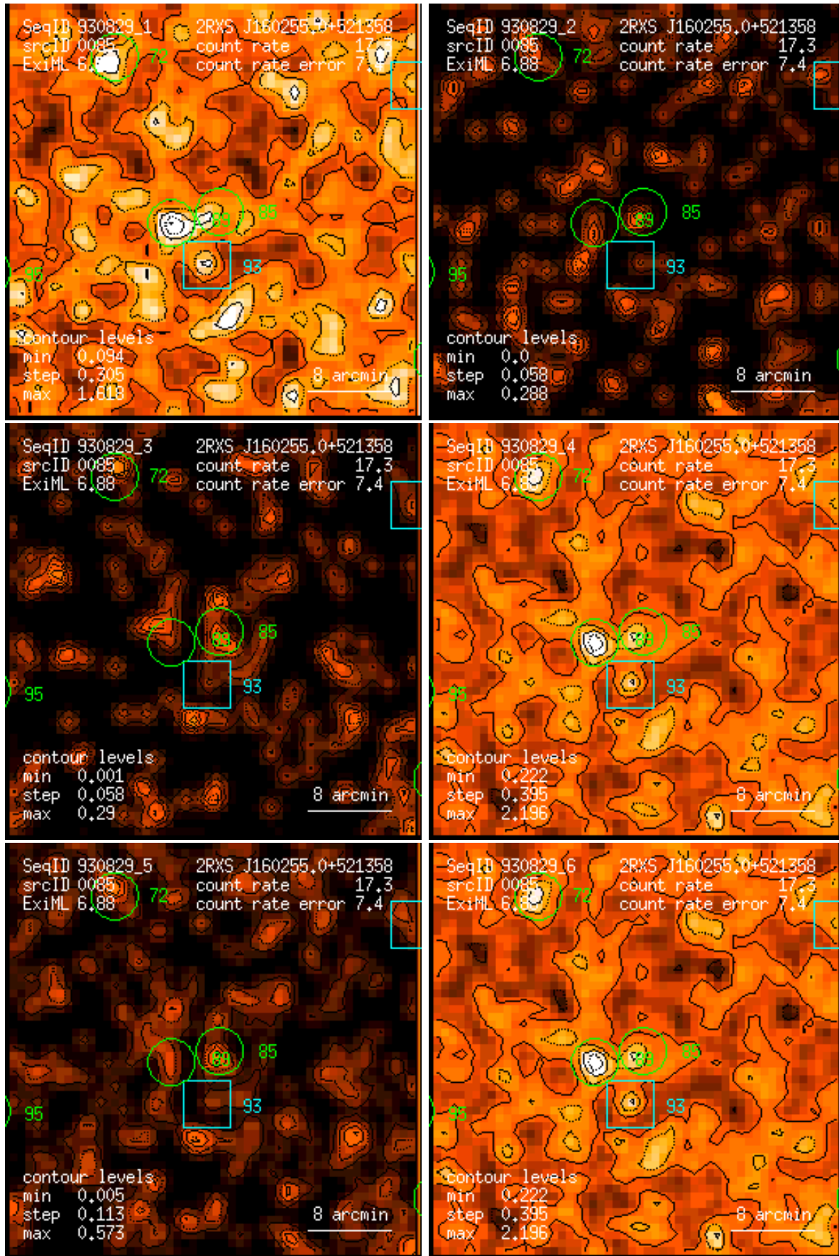
Figure 85: RASS 930829: detection 0085: band rate images, Gaussian filter: (1) PSPC channels 11 – 41, (2) 52 – 90, (3) 91 – 201, (4) 11 – 235, (5) 52 – 201, (6) 11 – 201. Broad band rates in counts/ks. Band rate contour levels in counts/ks/arcmin 2 .
