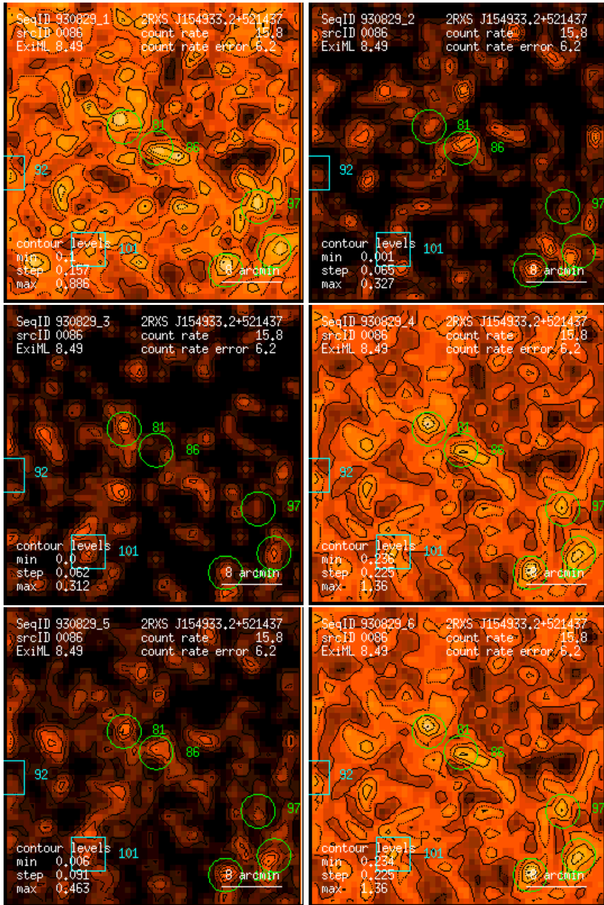
Figure 86: RASS 930829: detection 0086: band rate images, Gaussian filter: (1) PSPC channels 11 – 41, (2) 52 – 90, (3) 91 – 201, (4) 11 – 235, (5) 52 – 201, (6) 11 – 201. Broad band rates in counts/ks. Band rate contour levels in counts/ks/arcmin 2 .
