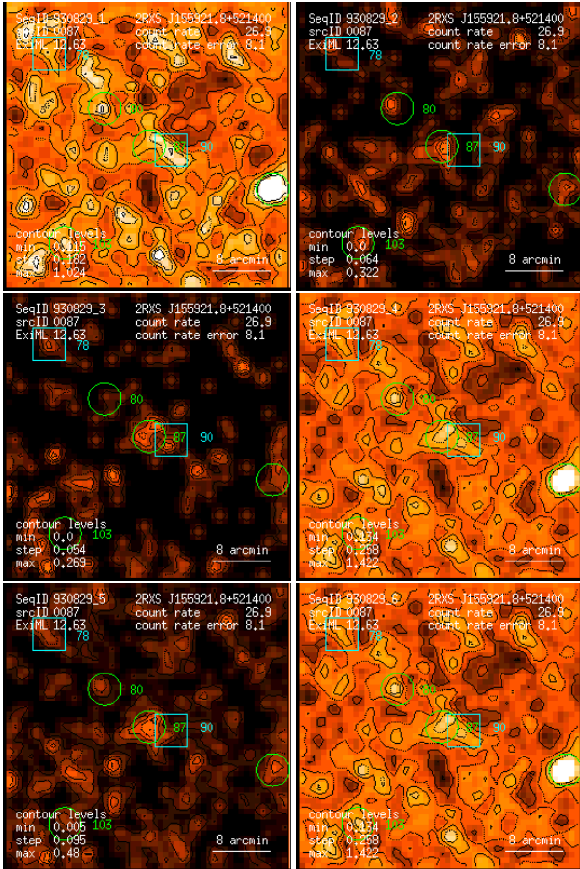
Figure 87: RASS 930829: detection 0087: band rate images, Gaussian filter: (1) PSPC channels 11 – 41, (2) 52 – 90, (3) 91 – 201, (4) 11 – 235, (5) 52 – 201, (6) 11 – 201. Broad band rates in counts/ks. Band rate contour levels in counts/ks/arcmin 2 .
