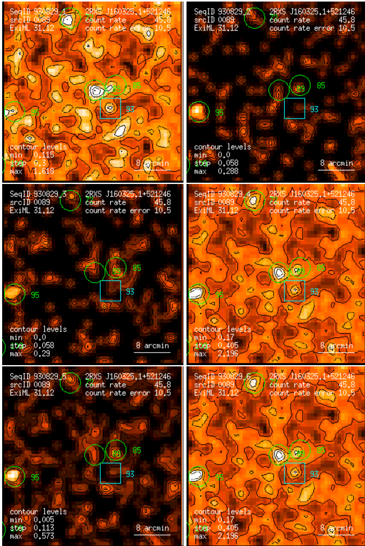
Figure 89: RASS 930829: detection 0089: band rate images, Gaussian filter: (1) PSPC channels 11 – 41, (2) 52 – 90, (3) 91 – 201, (4) 11 – 235, (5) 52 – 201, (6) 11 – 201. Broad band rates in counts/ks. Band rate contour levels in counts/ks/arcmin 2 .
