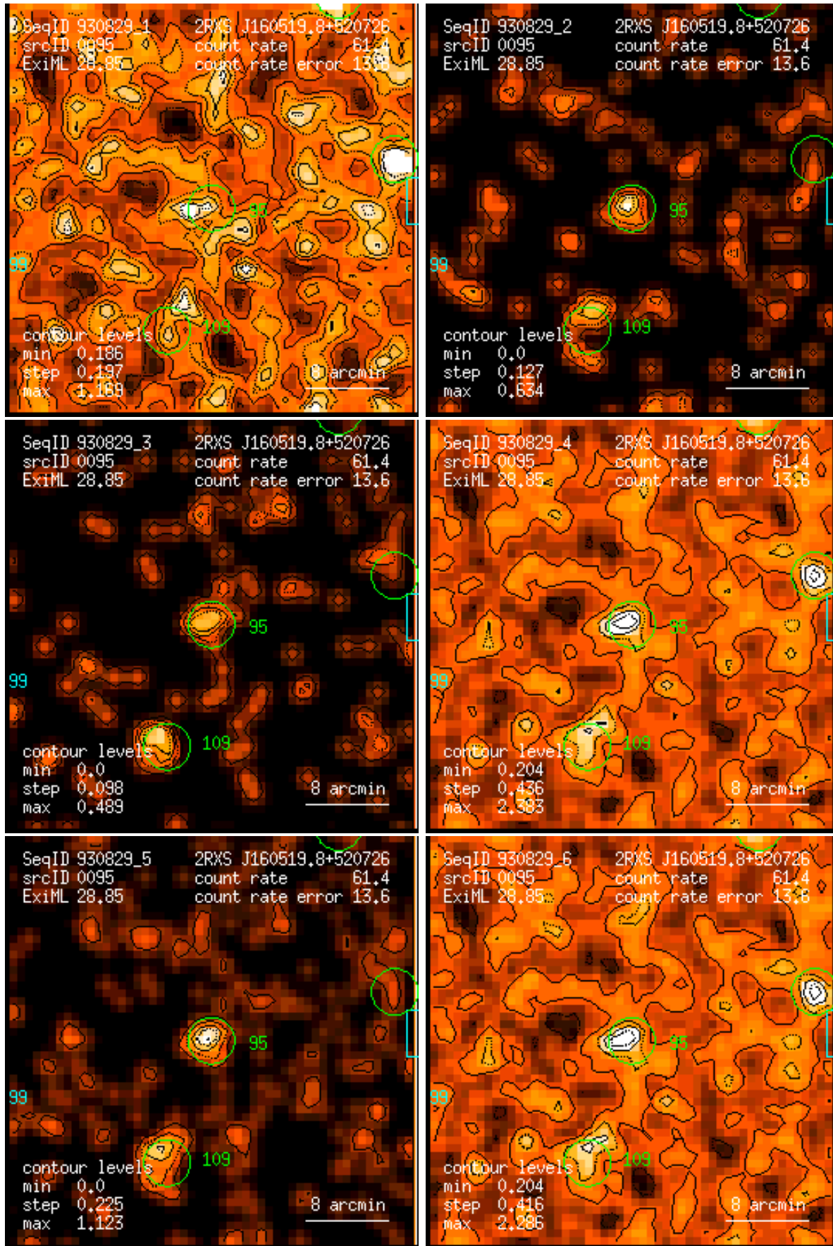
Figure 95: RASS 930829: detection 0095: band rate images, Gaussian filter: (1) PSPC channels 11 – 41, (2) 52 – 90, (3) 91 – 201, (4) 11 – 235, (5) 52 – 201, (6) 11 – 201. Broad band rates in counts/ks. Band rate contour levels in counts/ks/arcmin 2 .
