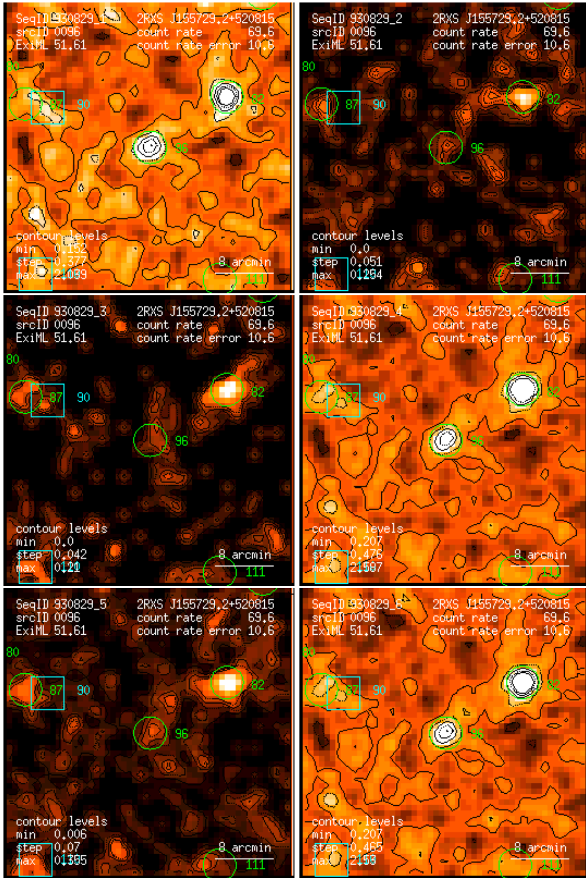
Figure 96: RASS 930829: detection 0096: band rate images, Gaussian filter: (1) PSPC channels 11 – 41, (2) 52 – 90, (3) 91 – 201, (4) 11 – 235, (5) 52 – 201, (6) 11 – 201. Broad band rates in counts/ks. Band rate contour levels in counts/ks/arcmin 2 .
