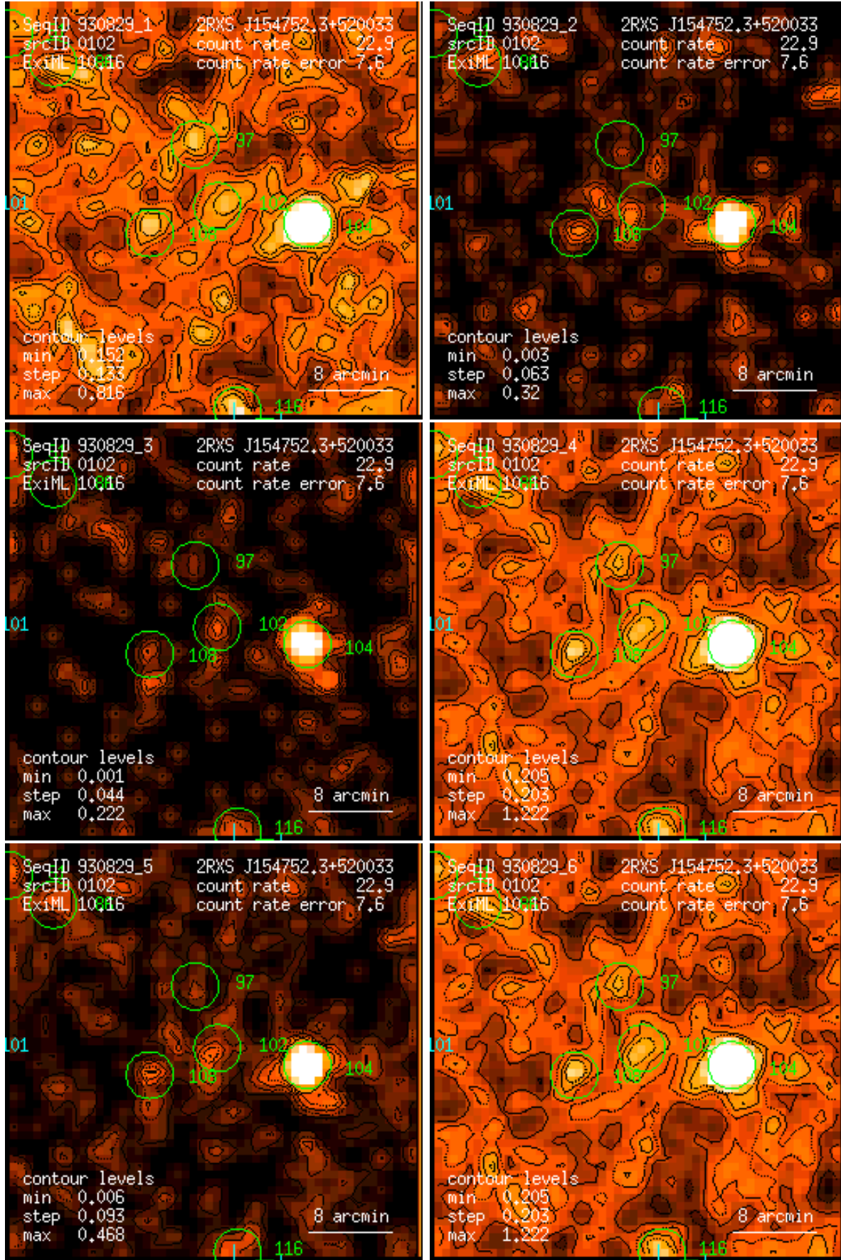
Figure 102: RASS 930829: detection 0102: band rate images, Gaussian filter: (1) PSPC channels 11 – 41, (2) 52 – 90, (3) 91 – 201, (4) 11 – 235, (5) 52 – 201, (6) 11 – 201. Broad band rates in counts/ks. Band rate contour levels in counts/ks/arcmin 2 .
