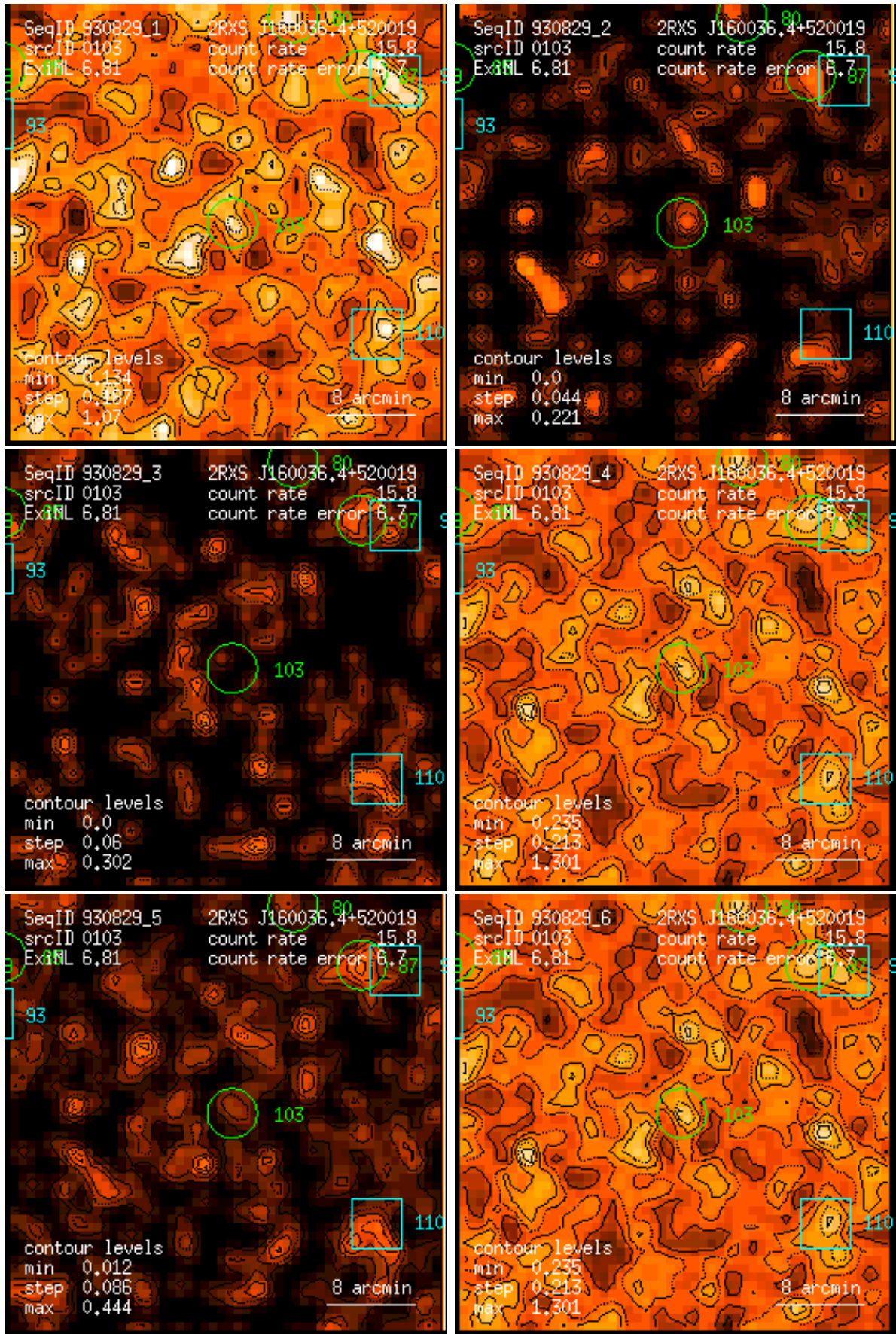
Figure 103: RASS 930829: detection 0103: band rate images, Gaussian filter: (1) PSPC channels 11 – 41, (2) 52 – 90, (3) 91 – 201, (4) 11 – 235, (5) 52 – 201, (6) 11 – 201. Broad band rates in counts/ks. Band rate contour levels in counts/ks/arcmin 2 .
