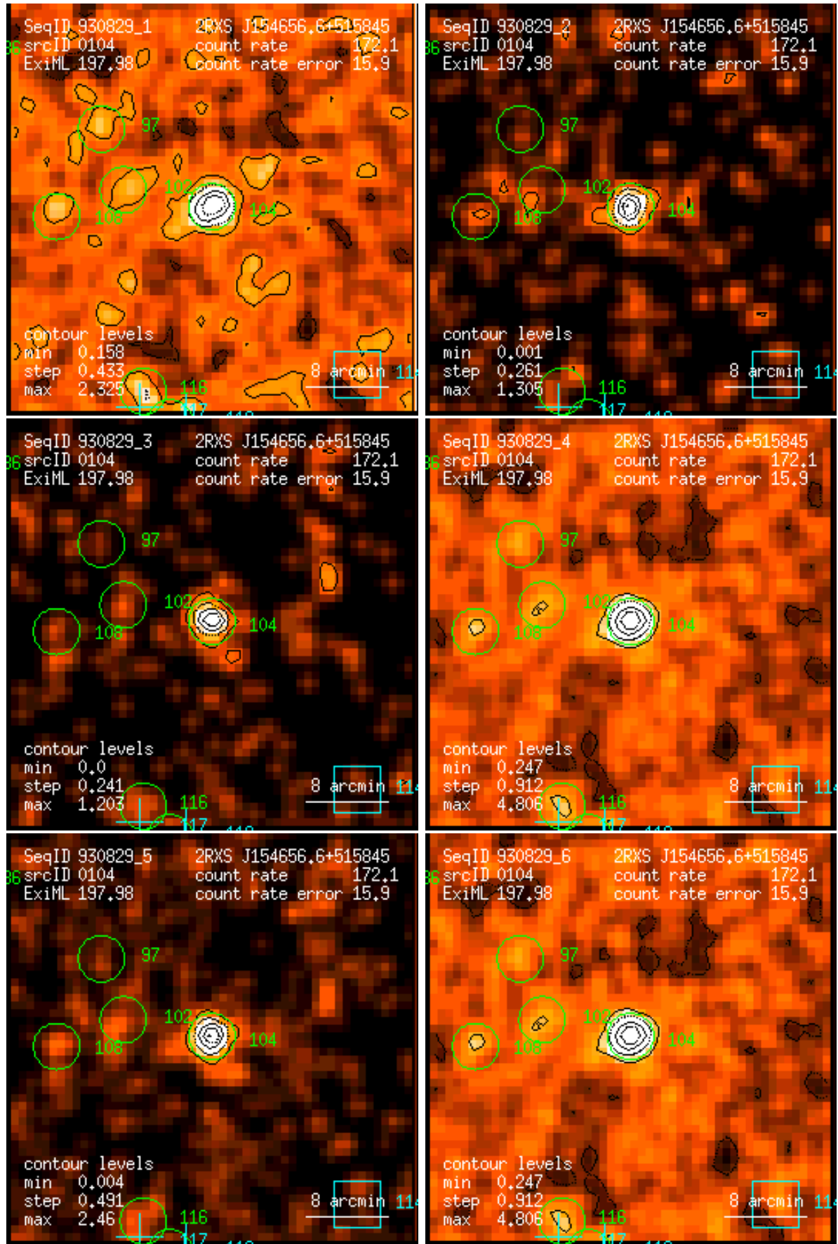
Figure 104: RASS 930829: detection 0104: band rate images, Gaussian filter: (1) PSPC channels 11 – 41, (2) 52 – 90, (3) 91 – 201, (4) 11 – 235, (5) 52 – 201, (6) 11 – 201. Broad band rates in counts/ks. Band rate contour levels in counts/ks/arcmin 2 .
