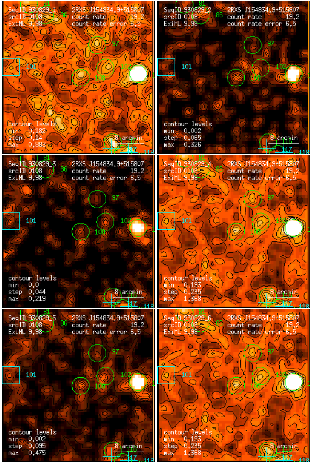
Figure 108: RASS 930829: detection 0108: band rate images, Gaussian filter: (1) PSPC channels 11 – 41, (2) 52 – 90, (3) 91 – 201, (4) 11 – 235, (5) 52 – 201, (6) 11 – 201. Broad band rates in counts/ks. Band rate contour levels in counts/ks/arcmin 2 .
