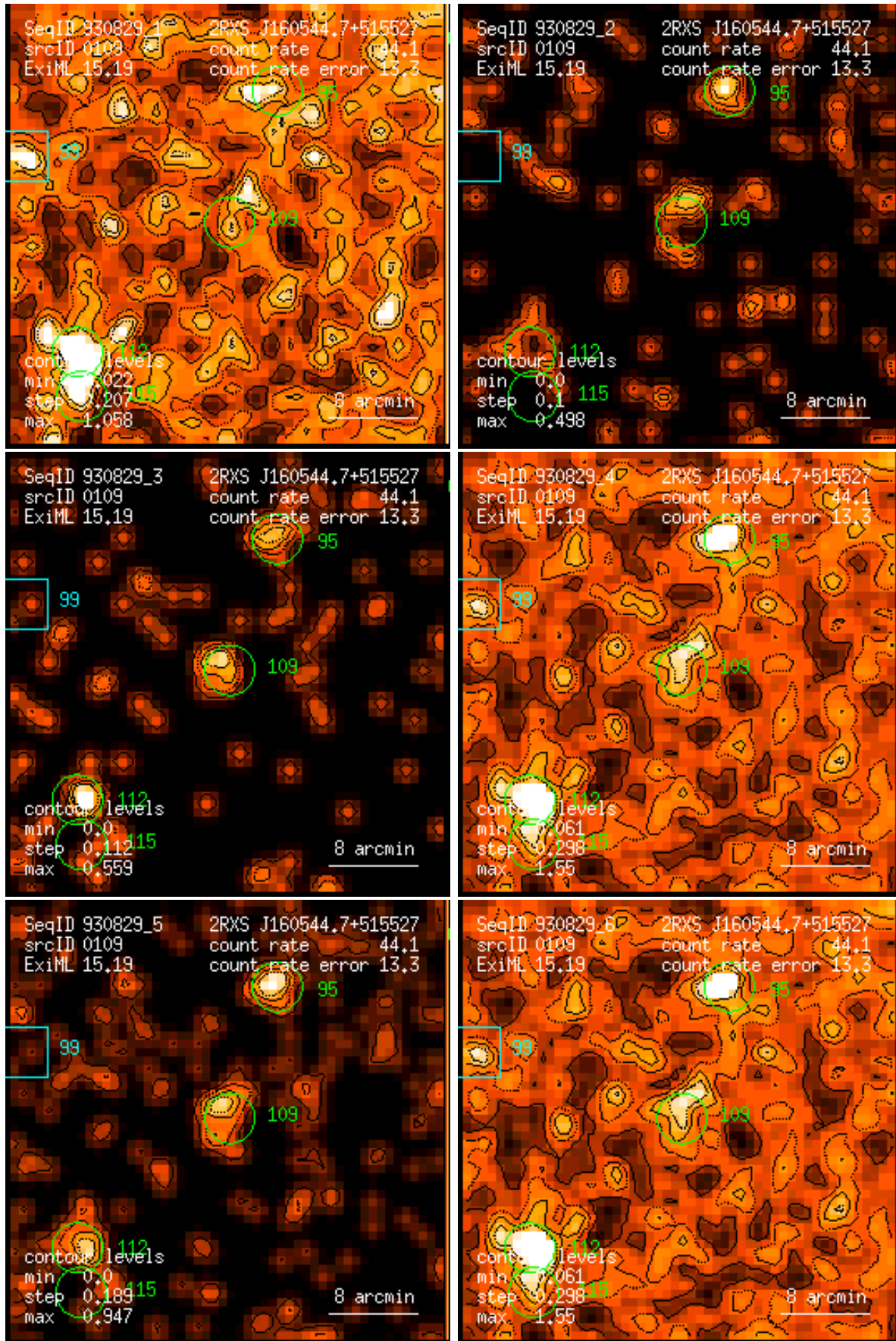
Figure 109: RASS 930829: detection 0109: band rate images, Gaussian filter: (1) PSPC channels 11 – 41, (2) 52 – 90, (3) 91 – 201, (4) 11 – 235, (5) 52 – 201, (6) 11 – 201. Broad band rates in counts/ks. Band rate contour levels in counts/ks/arcmin 2 .
