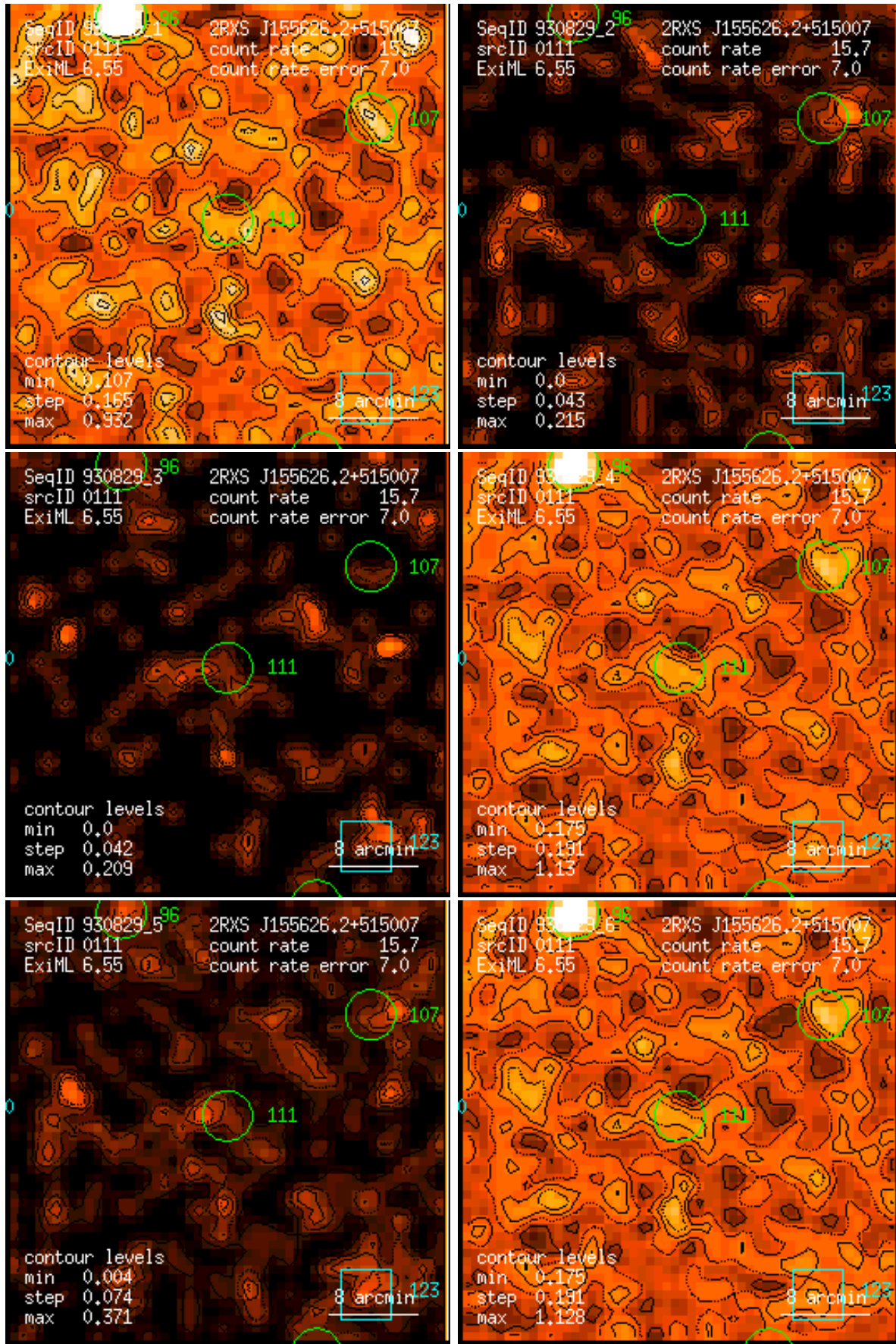
Figure 111: RASS 930829: detection 0111: band rate images, Gaussian filter: (1) PSPC channels 11 – 41, (2) 52 – 90, (3) 91 – 201, (4) 11 – 235, (5) 52 – 201, (6) 11 – 201. Broad band rates in counts/ks. Band rate contour levels in counts/ks/arcmin 2 .
