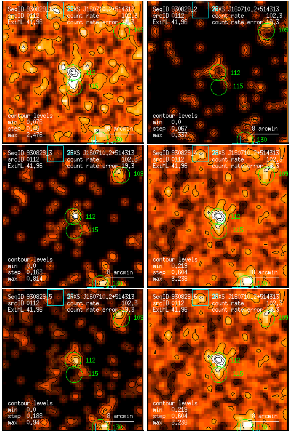
Figure 112: RASS 930829: detection 0112: band rate images, Gaussian filter: (1) PSPC channels 11 – 41, (2) 52 – 90, (3) 91 – 201, (4) 11 – 235, (5) 52 – 201, (6) 11 – 201. Broad band rates in counts/ks. Band rate contour levels in counts/ks/arcmin 2 .
