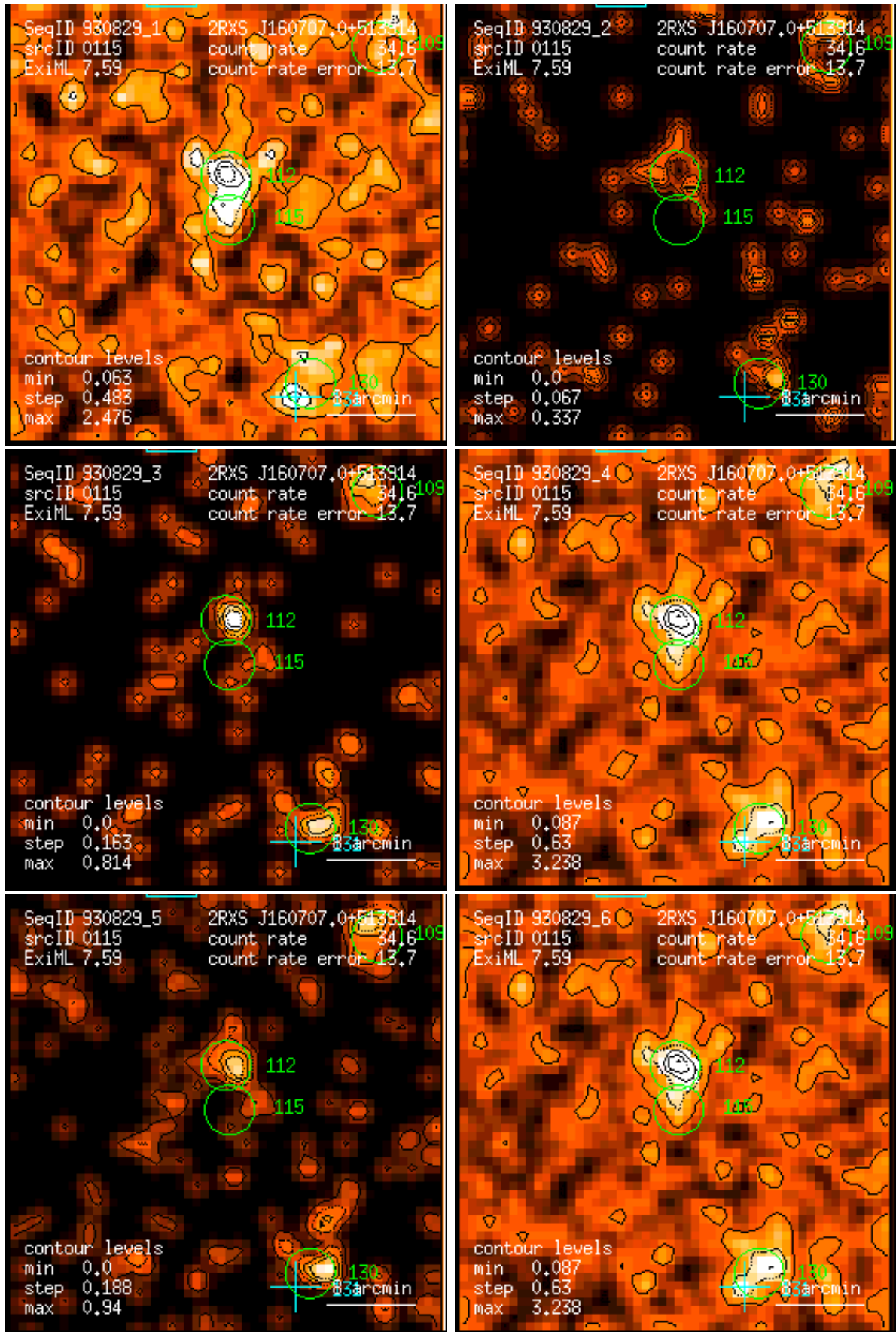
Figure 115: RASS 930829: detection 0115: band rate images, Gaussian filter: (1) PSPC channels 11 – 41, (2) 52 – 90, (3) 91 – 201, (4) 11 – 235, (5) 52 – 201, (6) 11 – 201. Broad band rates in counts/ks. Band rate contour levels in counts/ks/arcmin 2 .
