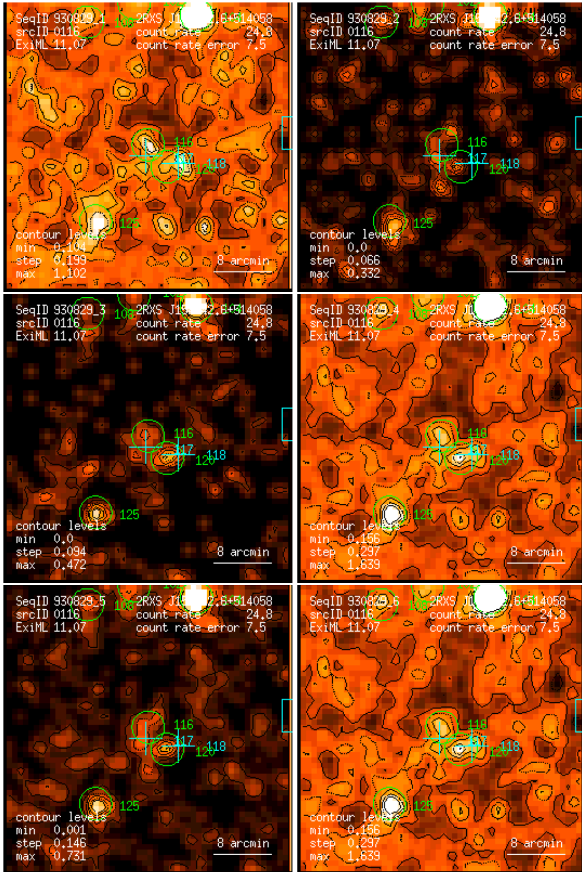
Figure 116: RASS 930829: detection 0116: band rate images, Gaussian filter: (1) PSPC channels 11 – 41, (2) 52 – 90, (3) 91 – 201, (4) 11 – 235, (5) 52 – 201, (6) 11 – 201. Broad band rates in counts/ks. Band rate contour levels in counts/ks/arcmin 2 .
