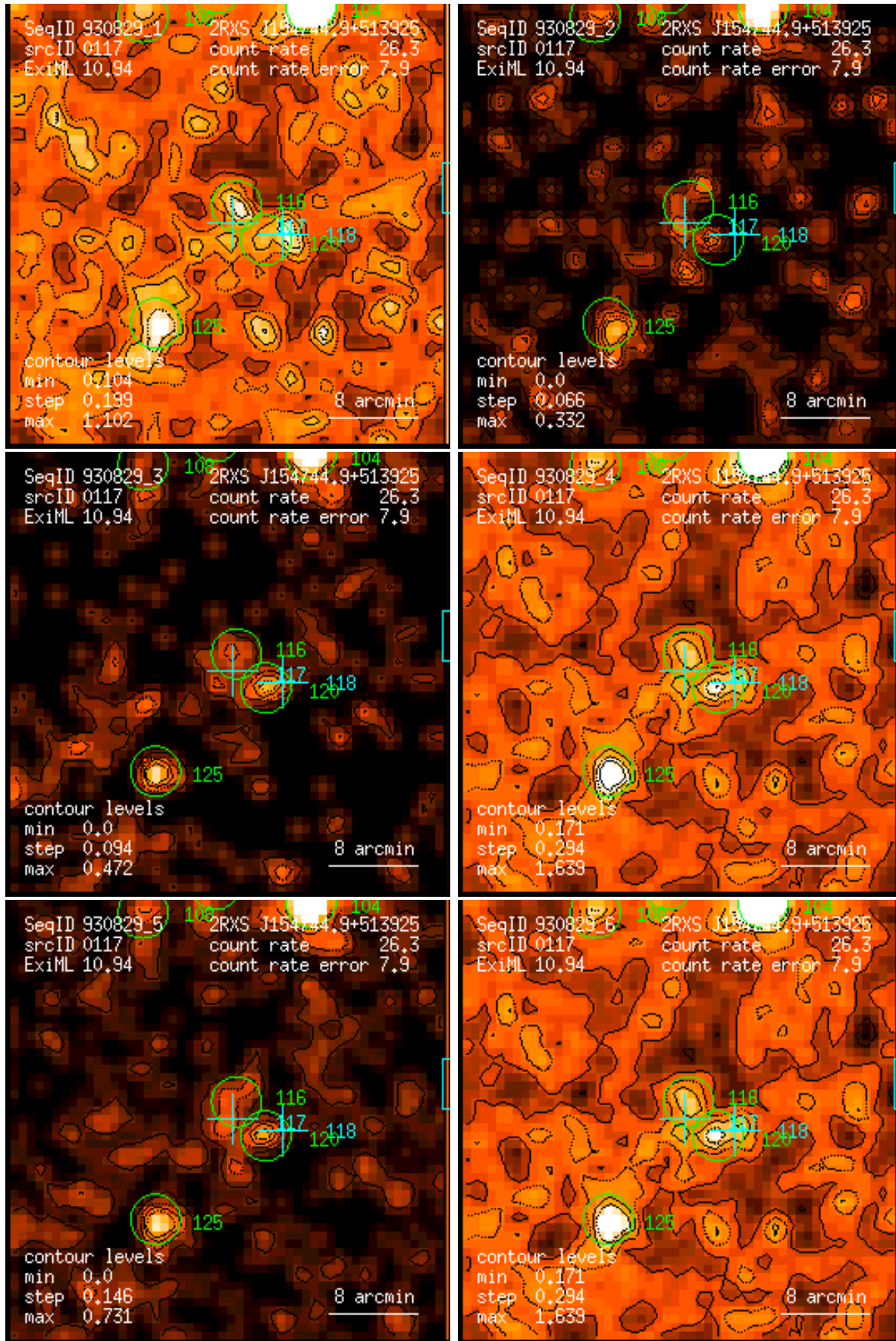
Figure 117: RASS 930829: detection 0117: band rate images, Gaussian filter: (1) PSPC channels 11 – 41, (2) 52 – 90, (3) 91 – 201, (4) 11 – 235, (5) 52 – 201, (6) 11 – 201. Broad band rates in counts/ks. Band rate contour levels in counts/ks/arcmin 2 .
