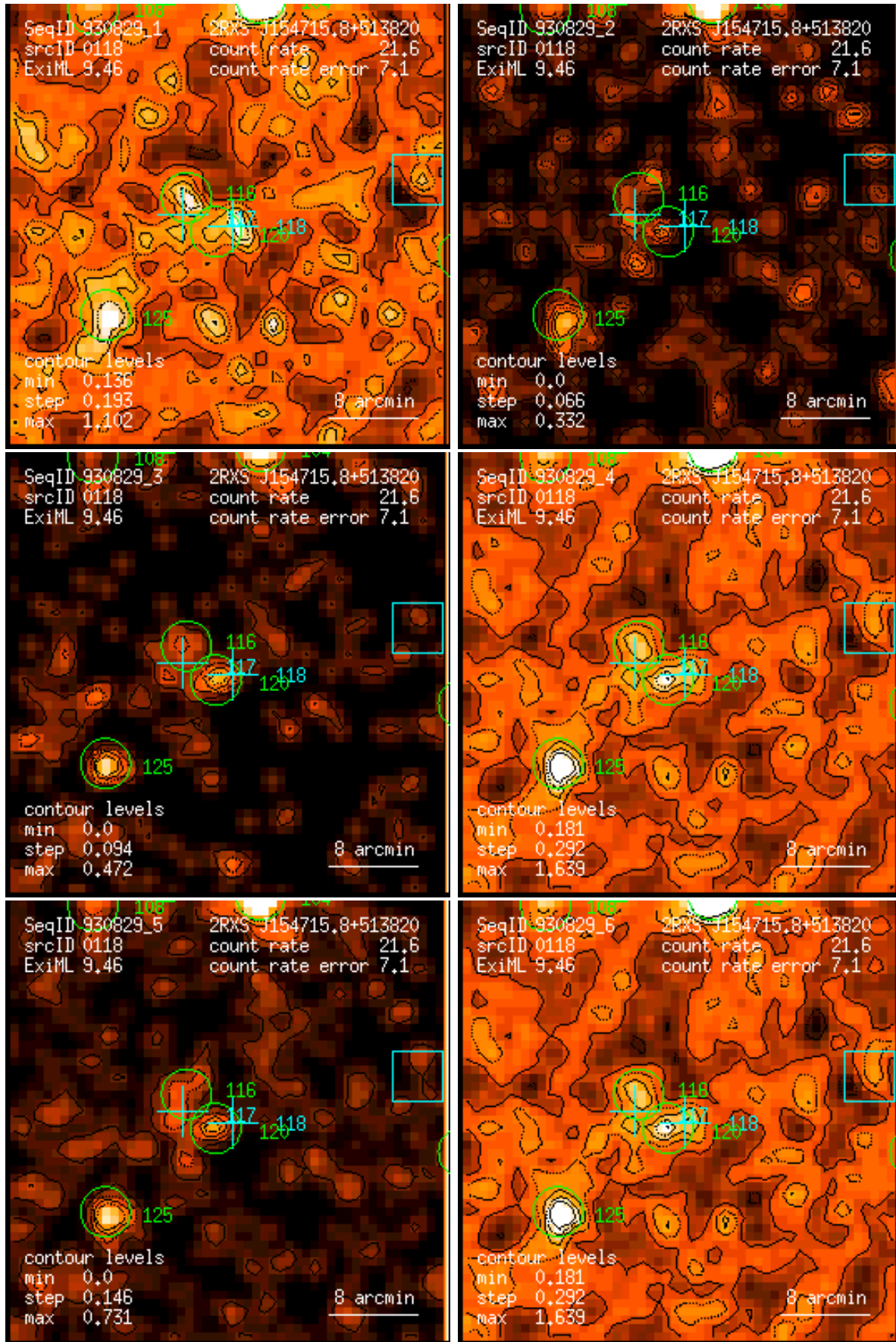
Figure 118: RASS 930829: detection 0118: band rate images, Gaussian filter: (1) PSPC channels 11 – 41, (2) 52 – 90, (3) 91 – 201, (4) 11 – 235, (5) 52 – 201, (6) 11 – 201. Broad band rates in counts/ks. Band rate contour levels in counts/ks/arcmin 2 .
