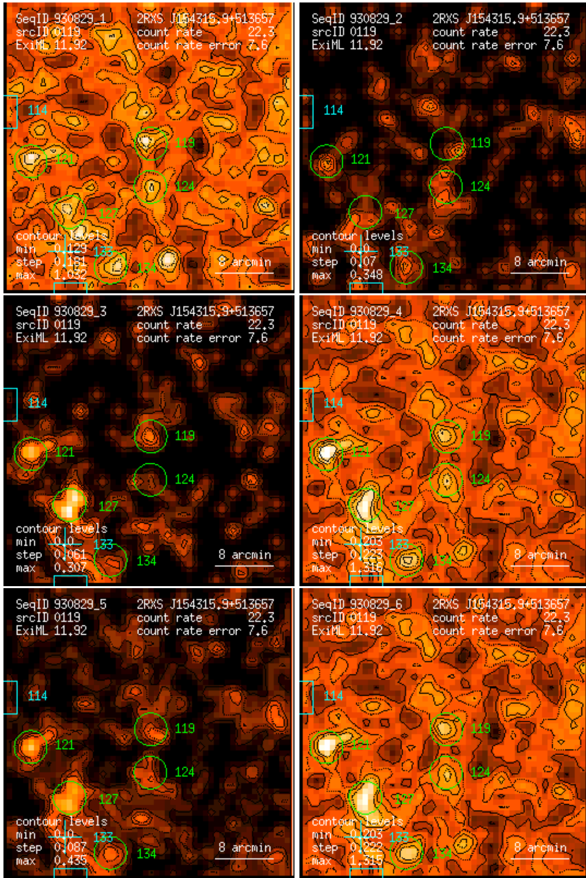
Figure 119: RASS 930829: detection 0119: band rate images, Gaussian filter: (1) PSPC channels 11 – 41, (2) 52 – 90, (3) 91 – 201, (4) 11 – 235, (5) 52 – 201, (6) 11 – 201. Broad band rates in counts/ks. Band rate contour levels in counts/ks/arcmin 2 .
