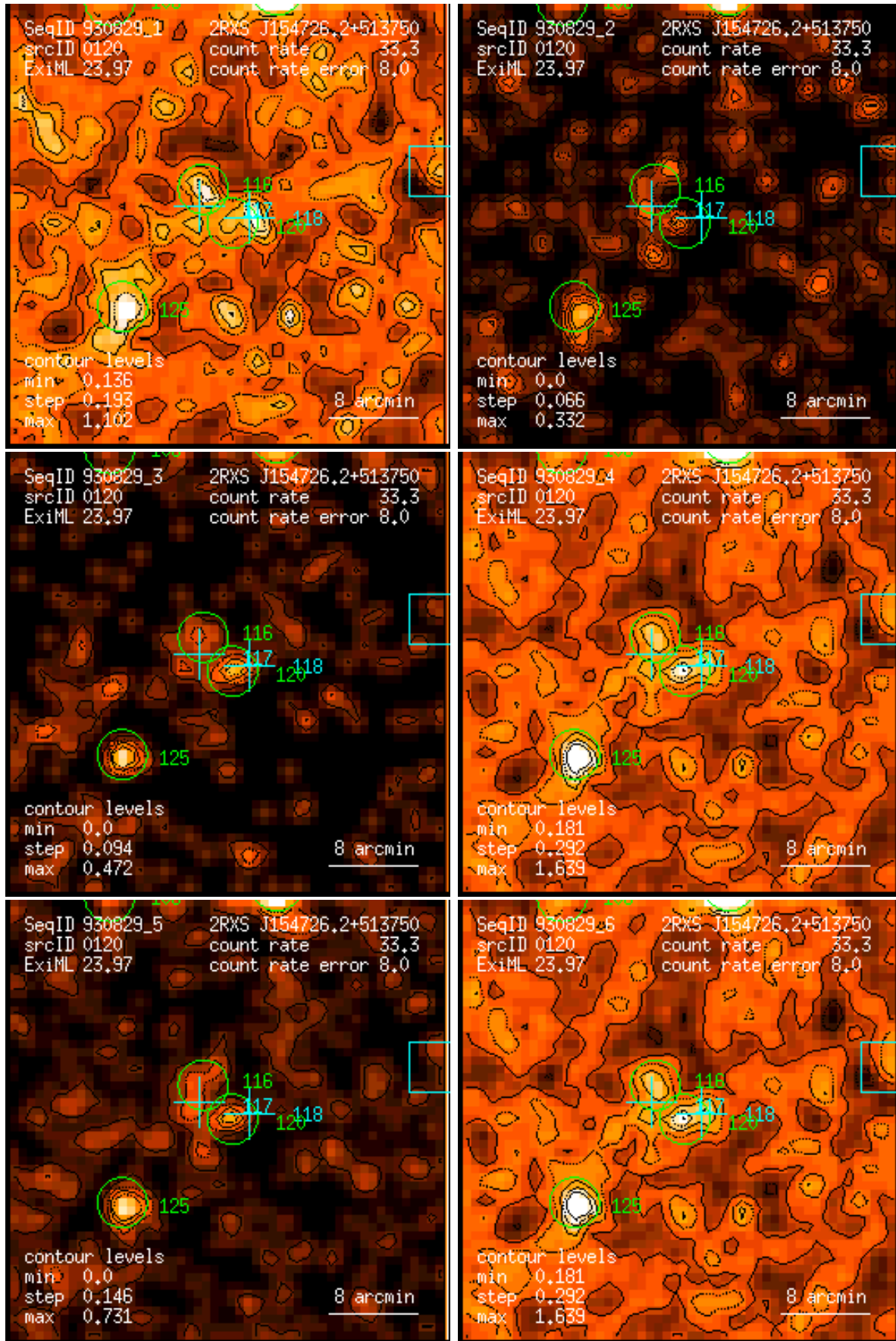
Figure 120: RASS 930829: detection 0120: band rate images, Gaussian filter: (1) PSPC channels 11 – 41, (2) 52 – 90, (3) 91 – 201, (4) 11 – 235, (5) 52 – 201, (6) 11 – 201. Broad band rates in counts/ks. Band rate contour levels in counts/ks/arcmin 2 .
