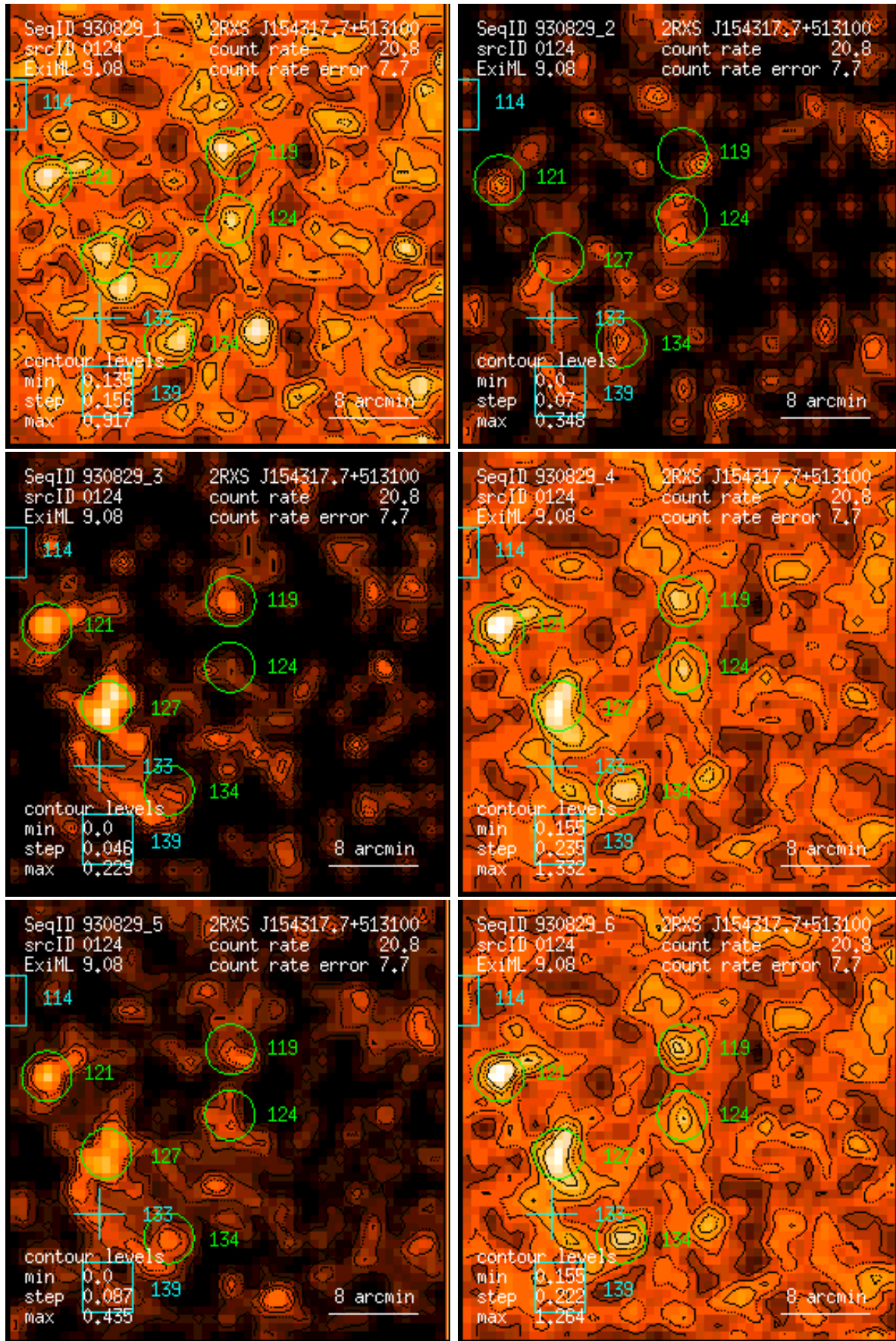
Figure 124: RASS 930829: detection 0124: band rate images, Gaussian filter: (1) PSPC channels 11 – 41, (2) 52 – 90, (3) 91 – 201, (4) 11 – 235, (5) 52 – 201, (6) 11 – 201. Broad band rates in counts/ks. Band rate contour levels in counts/ks/arcmin 2 .
