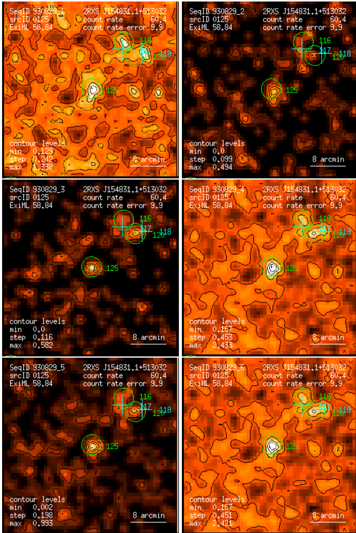
Figure 125: RASS 930829: detection 0125: band rate images, Gaussian filter: (1) PSPC channels 11 – 41, (2) 52 – 90, (3) 91 – 201, (4) 11 – 235, (5) 52 – 201, (6) 11 – 201. Broad band rates in counts/ks. Band rate contour levels in counts/ks/arcmin 2 .
