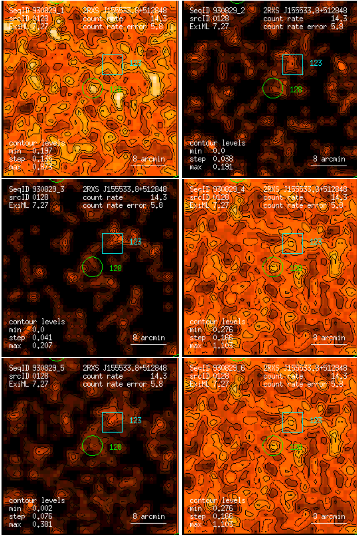
Figure 128: RASS 930829: detection 0128: band rate images, Gaussian filter: (1) PSPC channels 11 – 41, (2) 52 – 90, (3) 91 – 201, (4) 11 – 235, (5) 52 – 201, (6) 11 – 201. Broad band rates in counts/ks. Band rate contour levels in counts/ks/arcmin 2 .
