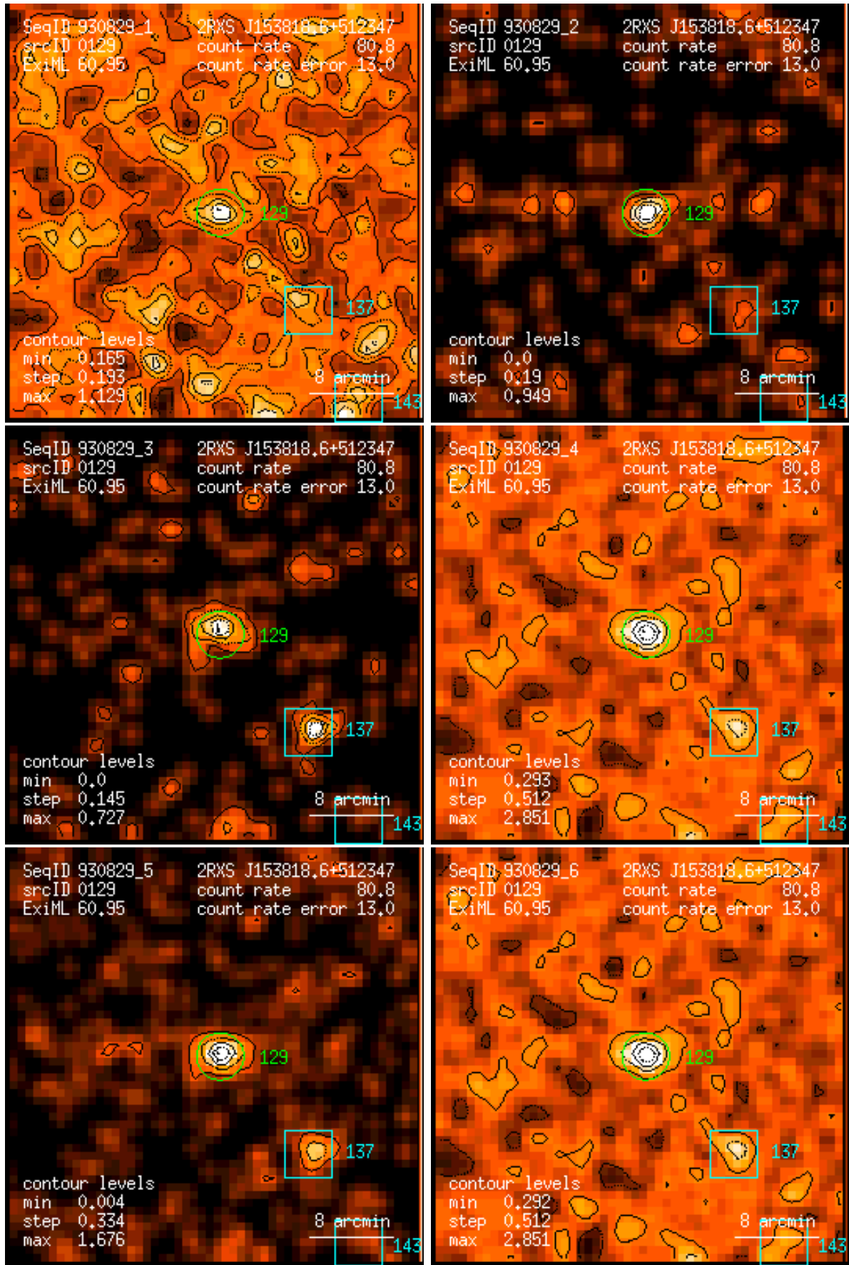
Figure 129: RASS 930829: detection 0129: band rate images, Gaussian filter: (1) PSPC channels 11 – 41, (2) 52 – 90, (3) 91 – 201, (4) 11 – 235, (5) 52 – 201, (6) 11 – 201. Broad band rates in counts/ks. Band rate contour levels in counts/ks/arcmin 2 .
