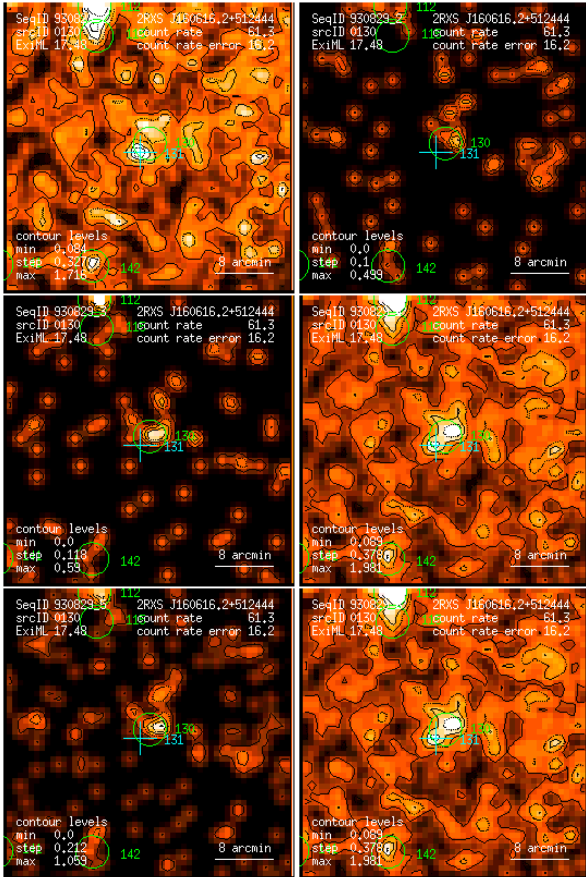
Figure 130: RASS 930829: detection 0130: band rate images, Gaussian filter: (1) PSPC channels 11 – 41, (2) 52 – 90, (3) 91 – 201, (4) 11 – 235, (5) 52 – 201, (6) 11 – 201. Broad band rates in counts/ks. Band rate contour levels in counts/ks/arcmin 2 .
