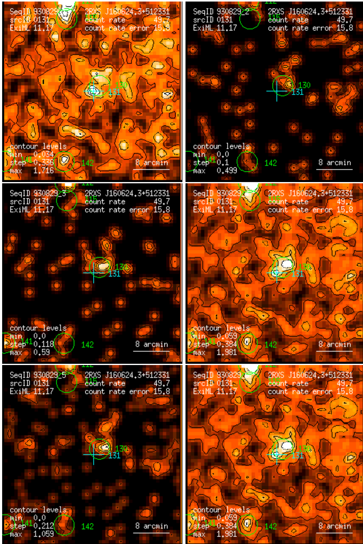
Figure 131: RASS 930829: detection 0131: band rate images, Gaussian filter: (1) PSPC channels 11 – 41, (2) 52 – 90, (3) 91 – 201, (4) 11 – 235, (5) 52 – 201, (6) 11 – 201. Broad band rates in counts/ks. Band rate contour levels in counts/ks/arcmin 2 .
