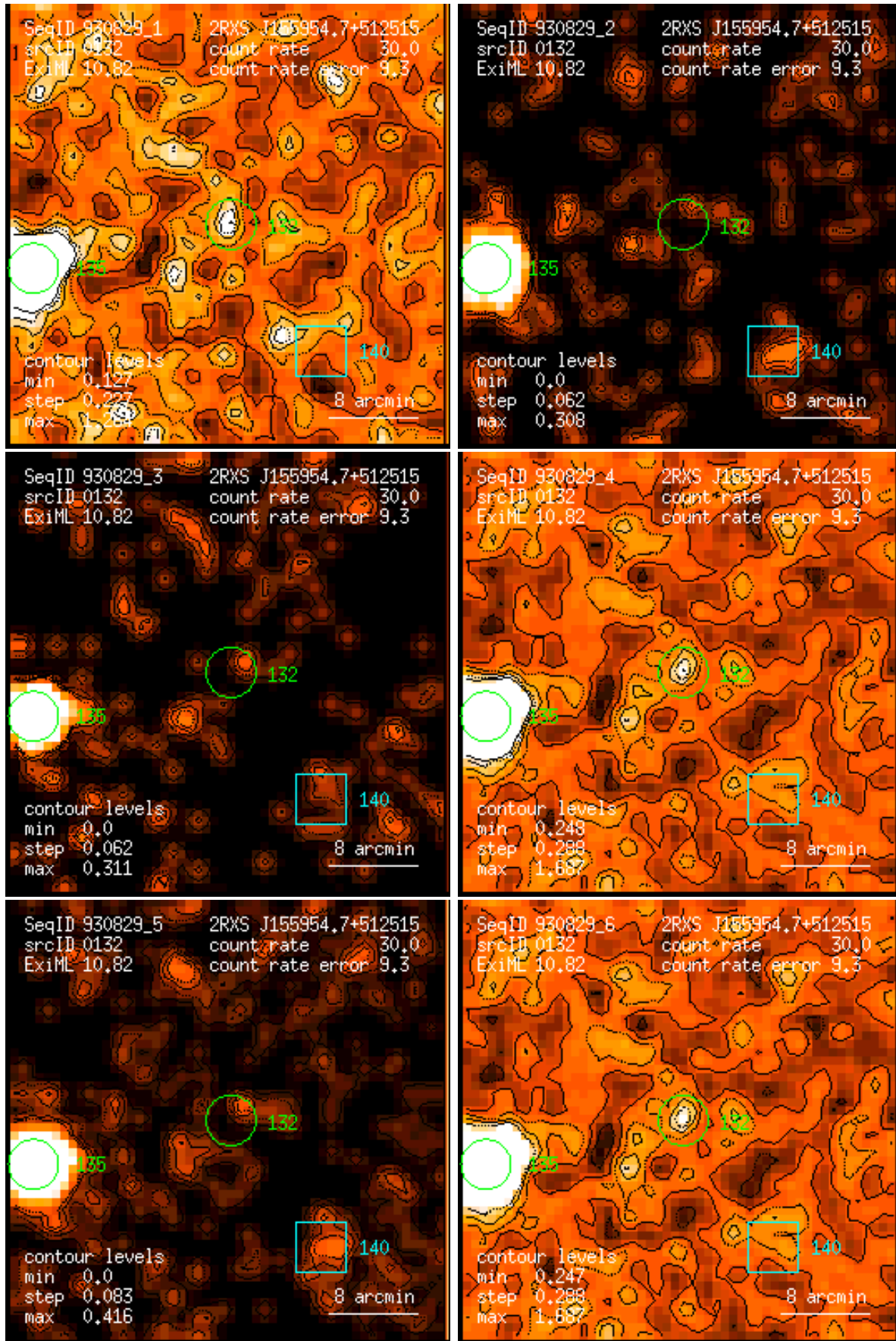
Figure 132: RASS 930829: detection 0132: band rate images, Gaussian filter: (1) PSPC channels 11 – 41, (2) 52 – 90, (3) 91 – 201, (4) 11 – 235, (5) 52 – 201, (6) 11 – 201. Broad band rates in counts/ks. Band rate contour levels in counts/ks/arcmin 2 .
