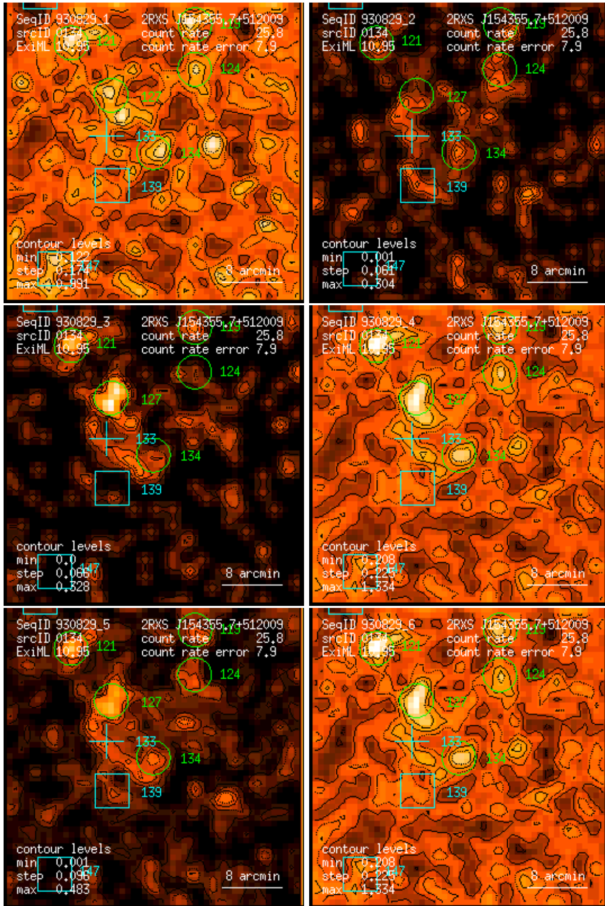
Figure 134: RASS 930829: detection 0134: band rate images, Gaussian filter: (1) PSPC channels 11 – 41, (2) 52 – 90, (3) 91 – 201, (4) 11 – 235, (5) 52 – 201, (6) 11 – 201. Broad band rates in counts/ks. Band rate contour levels in counts/ks/arcmin 2 .
