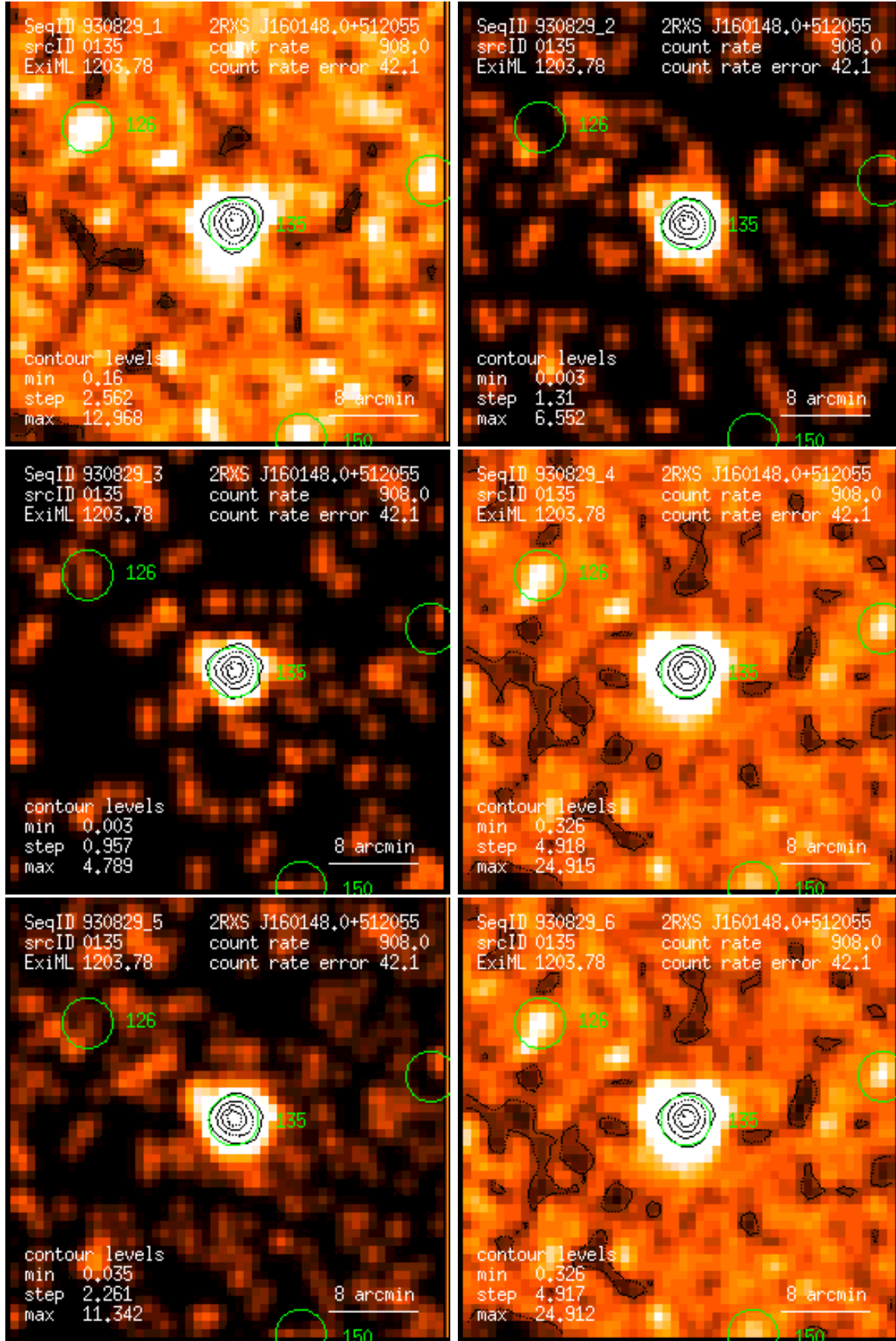
Figure 135: RASS 930829: detection 0135: band rate images, Gaussian filter: (1) PSPC channels 11 – 41, (2) 52 – 90, (3) 91 – 201, (4) 11 – 235, (5) 52 – 201, (6) 11 – 201. Broad band rates in counts/ks. Band rate contour levels in counts/ks/arcmin 2 .
