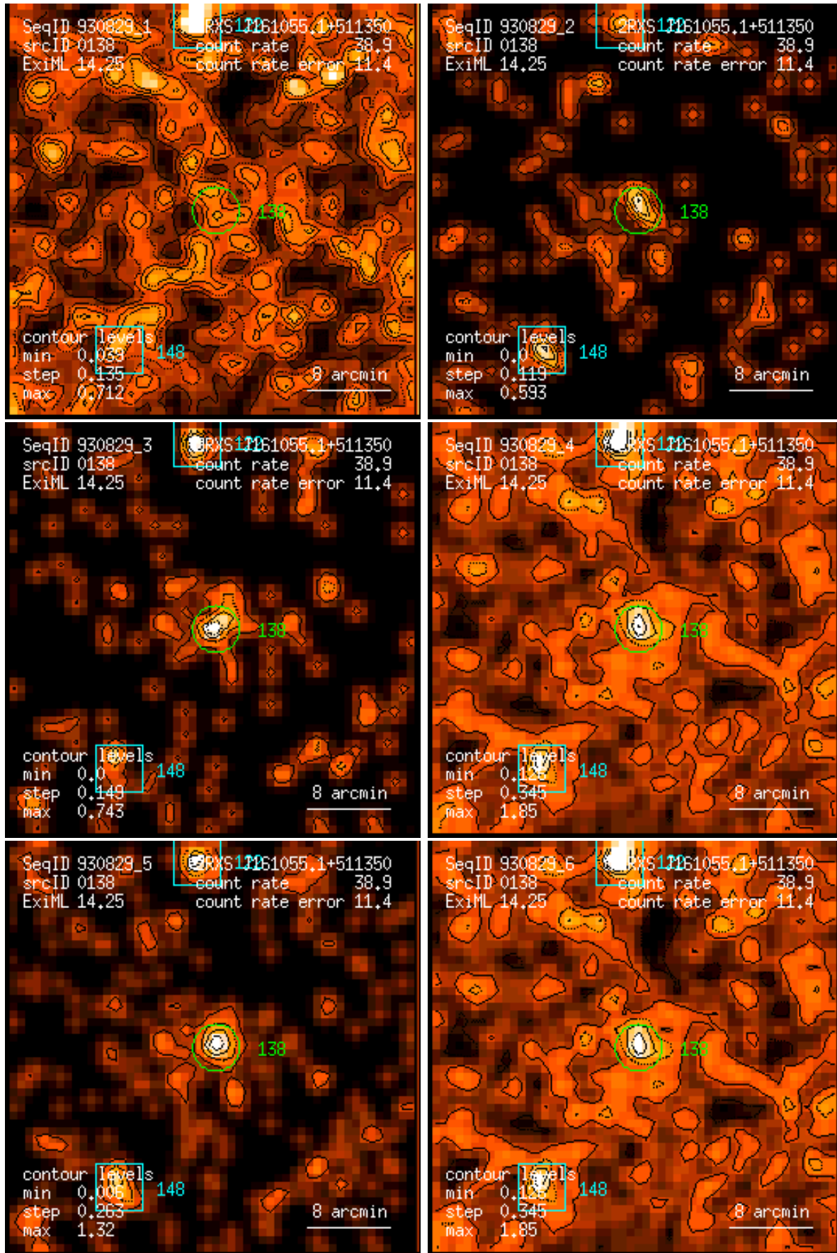
Figure 138: RASS 930829: detection 0138: band rate images, Gaussian filter: (1) PSPC channels 11 – 41, (2) 52 – 90, (3) 91 – 201, (4) 11 – 235, (5) 52 – 201, (6) 11 – 201. Broad band rates in counts/ks. Band rate contour levels in counts/ks/arcmin 2 .
