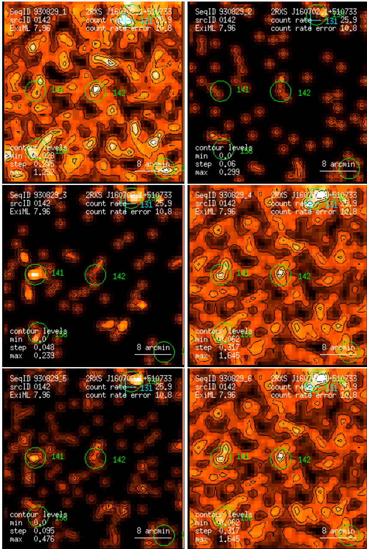
Figure 142: RASS 930829: detection 0142: band rate images, Gaussian filter: (1) PSPC channels 11 – 41, (2) 52 – 90, (3) 91 – 201, (4) 11 – 235, (5) 52 – 201, (6) 11 – 201. Broad band rates in counts/ks. Band rate contour levels in counts/ks/arcmin 2 .
