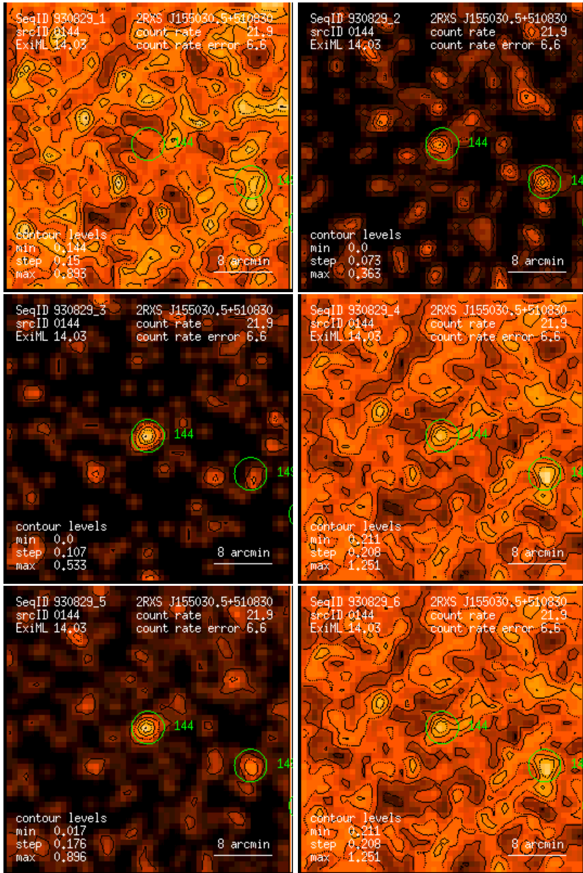
Figure 144: RASS 930829: detection 0144: band rate images, Gaussian filter: (1) PSPC channels 11 – 41, (2) 52 – 90, (3) 91 – 201, (4) 11 – 235, (5) 52 – 201, (6) 11 – 201. Broad band rates in counts/ks. Band rate contour levels in counts/ks/arcmin 2 .
