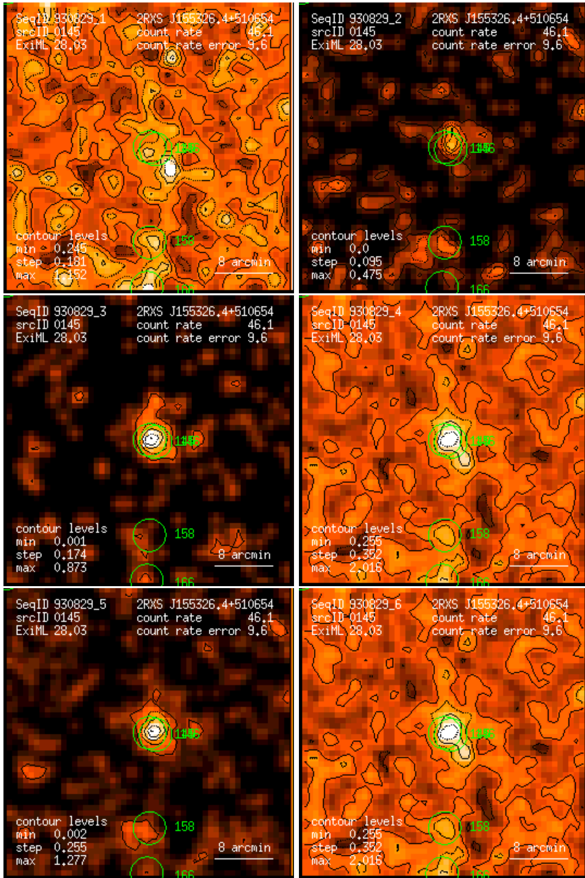
Figure 145: RASS 930829: detection 0145: band rate images, Gaussian filter: (1) PSPC channels 11 – 41, (2) 52 – 90, (3) 91 – 201, (4) 11 – 235, (5) 52 – 201, (6) 11 – 201. Broad band rates in counts/ks. Band rate contour levels in counts/ks/arcmin 2 .
