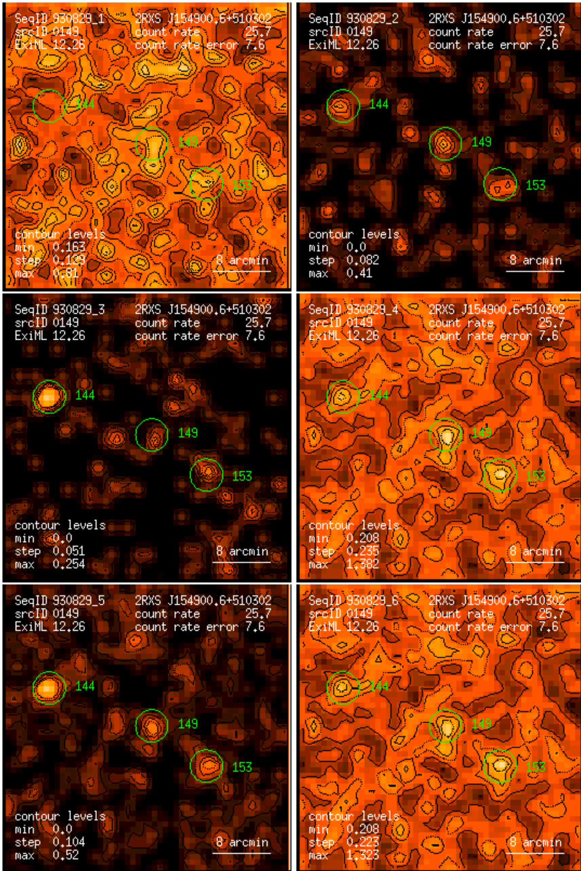
Figure 149: RASS 930829: detection 0149: band rate images, Gaussian filter: (1) PSPC channels 11 – 41, (2) 52 – 90, (3) 91 – 201, (4) 11 – 235, (5) 52 – 201, (6) 11 – 201. Broad band rates in counts/ks. Band rate contour levels in counts/ks/arcmin 2 .
