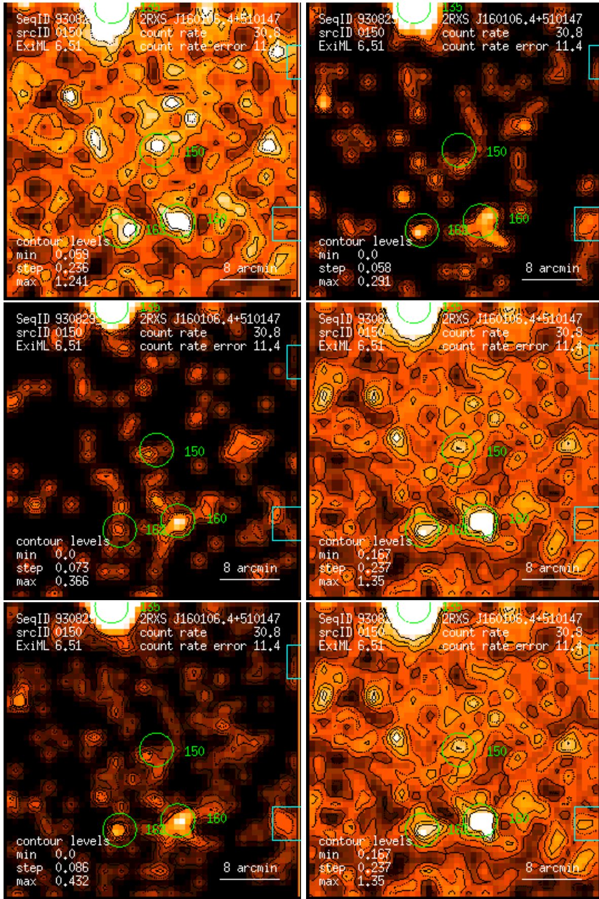
Figure 150: RASS 930829: detection 0150: band rate images, Gaussian filter: (1) PSPC channels 11 – 41, (2) 52 – 90, (3) 91 – 201, (4) 11 – 235, (5) 52 – 201, (6) 11 – 201. Broad band rates in counts/ks. Band rate contour levels in counts/ks/arcmin 2 .
