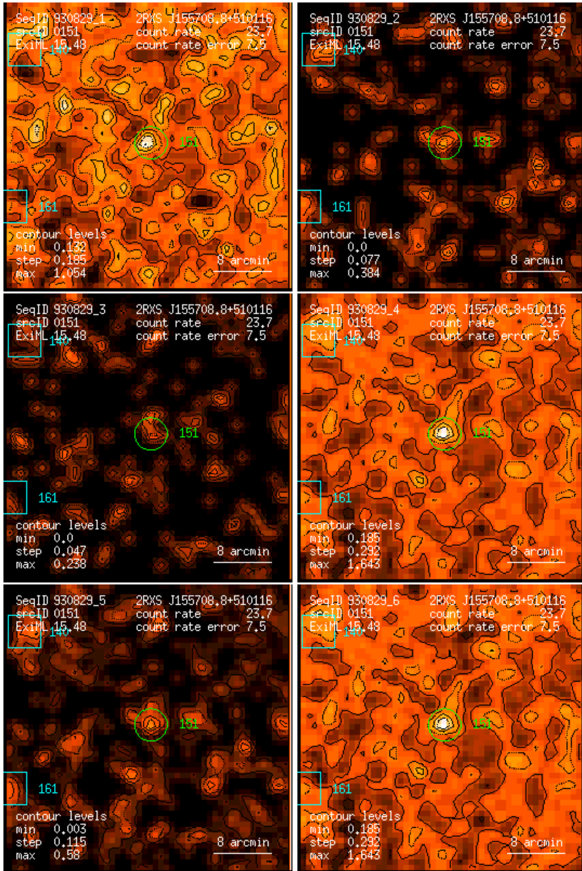
Figure 151: RASS 930829: detection 0151: band rate images, Gaussian filter: (1) PSPC channels 11 – 41, (2) 52 – 90, (3) 91 – 201, (4) 11 – 235, (5) 52 – 201, (6) 11 – 201. Broad band rates in counts/ks. Band rate contour levels in counts/ks/arcmin 2 .
