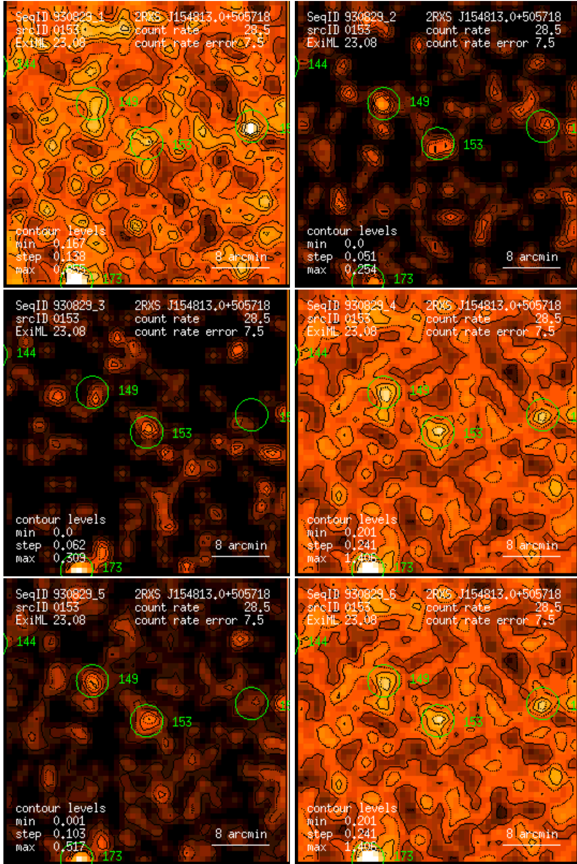
Figure 153: RASS 930829: detection 0153: band rate images, Gaussian filter: (1) PSPC channels 11 – 41, (2) 52 – 90, (3) 91 – 201, (4) 11 – 235, (5) 52 – 201, (6) 11 – 201. Broad band rates in counts/ks. Band rate contour levels in counts/ks/arcmin 2 .
