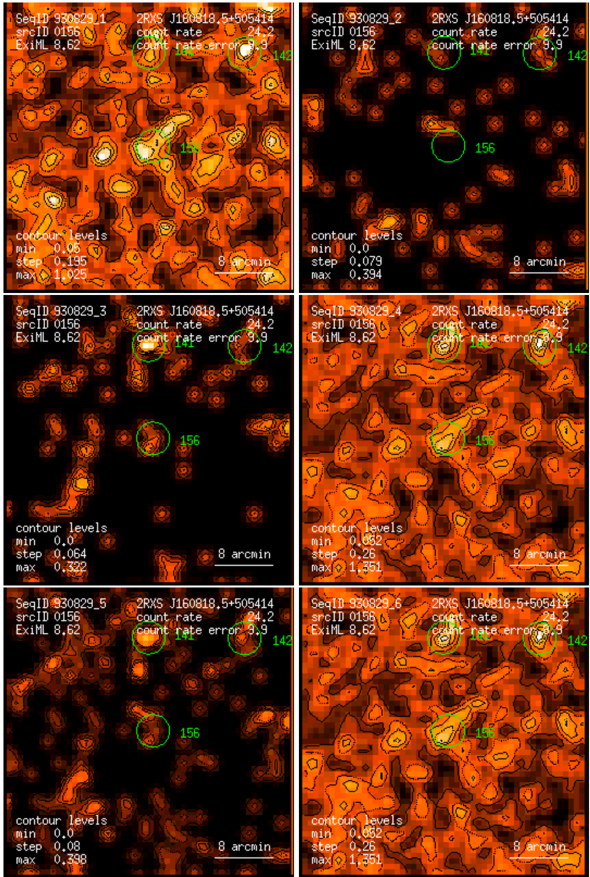
Figure 156: RASS 930829: detection 0156: band rate images, Gaussian filter: (1) PSPC channels 11 – 41, (2) 52 – 90, (3) 91 – 201, (4) 11 – 235, (5) 52 – 201, (6) 11 – 201. Broad band rates in counts/ks. Band rate contour levels in counts/ks/arcmin 2 .
