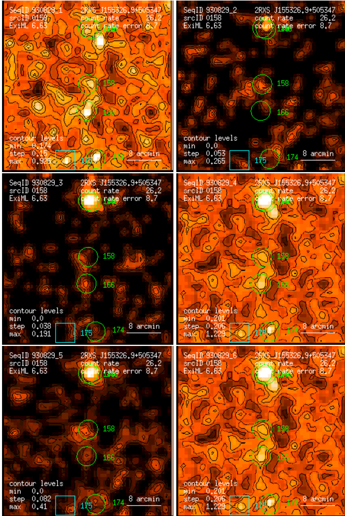
Figure 158: RASS 930829: detection 0158: band rate images, Gaussian filter: (1) PSPC channels 11 – 41, (2) 52 – 90, (3) 91 – 201, (4) 11 – 235, (5) 52 – 201, (6) 11 – 201. Broad band rates in counts/ks. Band rate contour levels in counts/ks/arcmin 2 .
