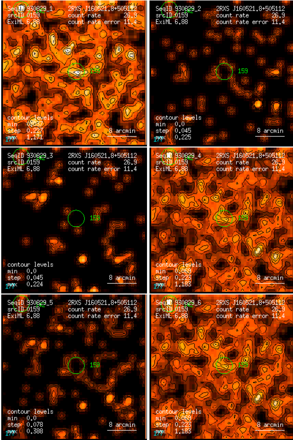
Figure 159: RASS 930829: detection 0159: band rate images, Gaussian filter: (1) PSPC channels 11 – 41, (2) 52 – 90, (3) 91 – 201, (4) 11 – 235, (5) 52 – 201, (6) 11 – 201. Broad band rates in counts/ks. Band rate contour levels in counts/ks/arcmin 2 .
