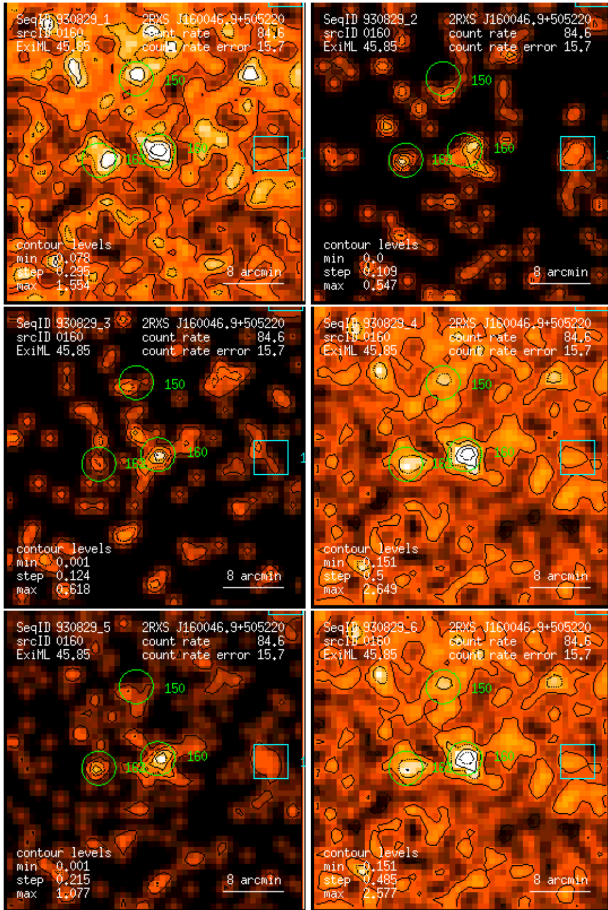
Figure 160: RASS 930829: detection 0160: band rate images, Gaussian filter: (1) PSPC channels 11 – 41, (2) 52 – 90, (3) 91 – 201, (4) 11 – 235, (5) 52 – 201, (6) 11 – 201. Broad band rates in counts/ks. Band rate contour levels in counts/ks/arcmin 2 .
