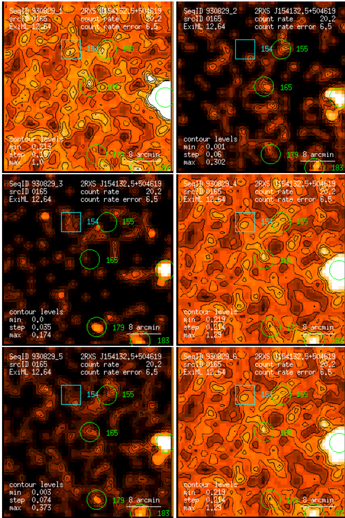
Figure 165: RASS 930829: detection 0165: band rate images, Gaussian filter: (1) PSPC channels 11 – 41, (2) 52 – 90, (3) 91 – 201, (4) 11 – 235, (5) 52 – 201, (6) 11 – 201. Broad band rates in counts/ks. Band rate contour levels in counts/ks/arcmin 2 .
