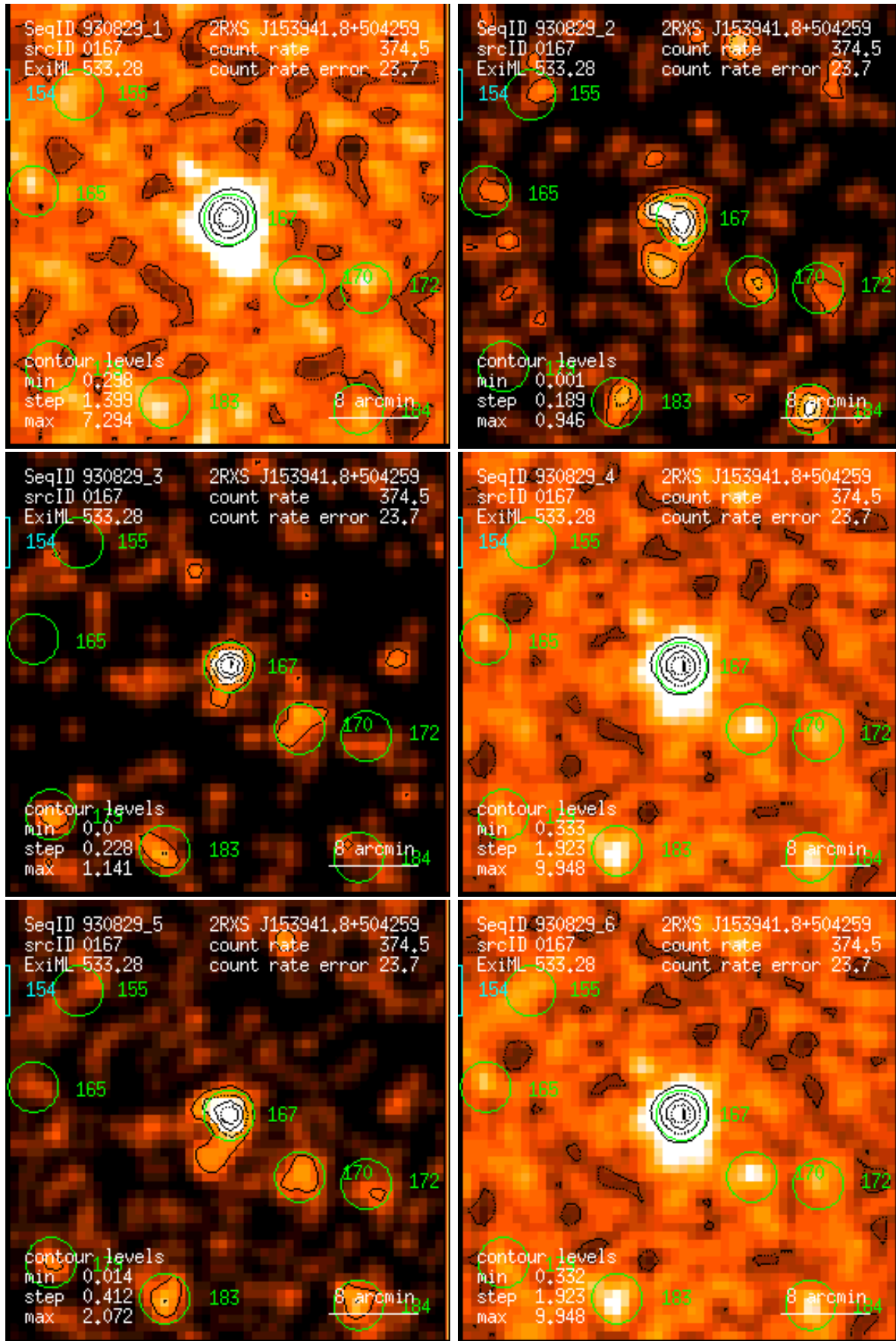
Figure 167: RASS 930829: detection 0167: band rate images, Gaussian filter: (1) PSPC channels 11 – 41, (2) 52 – 90, (3) 91 – 201, (4) 11 – 235, (5) 52 – 201, (6) 11 – 201. Broad band rates in counts/ks. Band rate contour levels in counts/ks/arcmin 2 .
