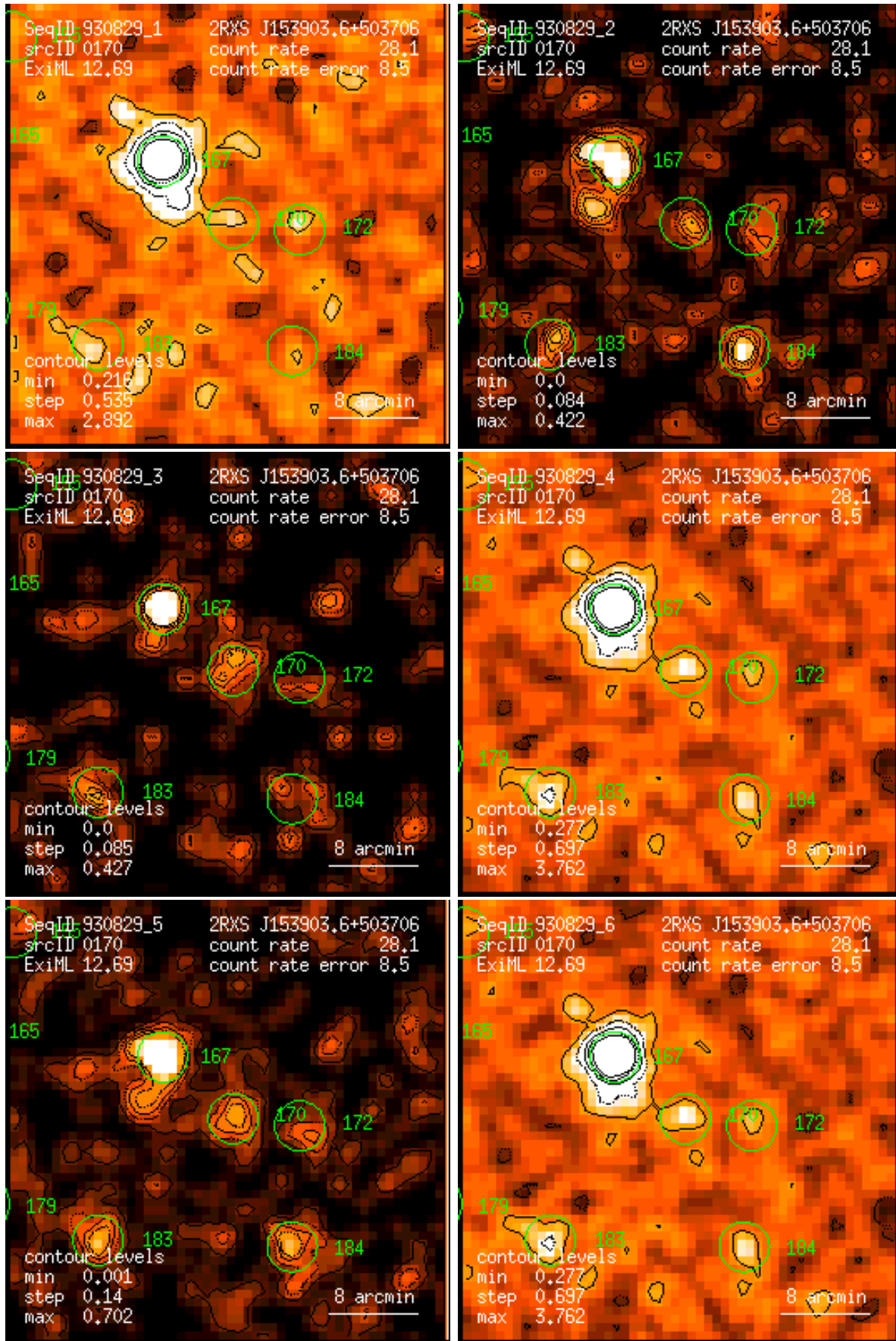
Figure 170: RASS 930829: detection 0170: band rate images, Gaussian filter: (1) PSPC channels 11 – 41, (2) 52 – 90, (3) 91 – 201, (4) 11 – 235, (5) 52 – 201, (6) 11 – 201. Broad band rates in counts/ks. Band rate contour levels in counts/ks/arcmin 2 .
