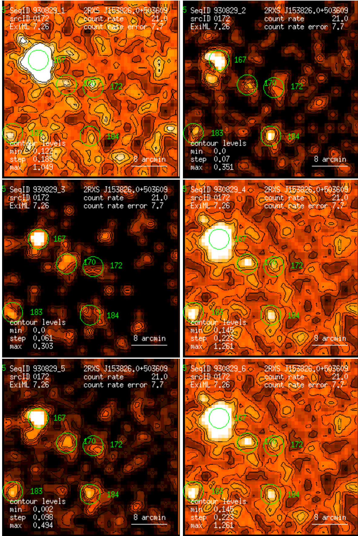
Figure 172: RASS 930829: detection 0172: band rate images, Gaussian filter: (1) PSPC channels 11 – 41, (2) 52 – 90, (3) 91 – 201, (4) 11 – 235, (5) 52 – 201, (6) 11 – 201. Broad band rates in counts/ks. Band rate contour levels in counts/ks/arcmin 2 .
