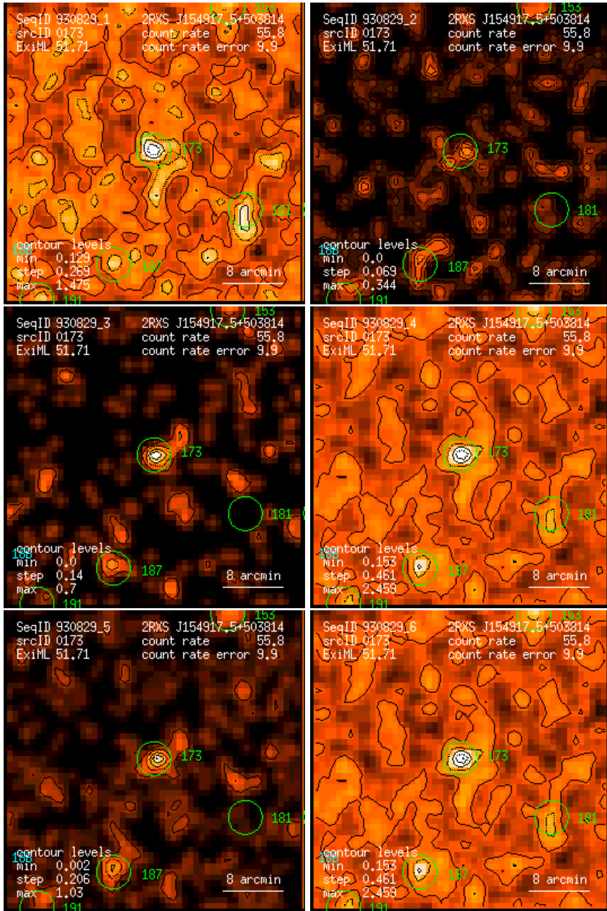
Figure 173: RASS 930829: detection 0173: band rate images, Gaussian filter: (1) PSPC channels 11 – 41, (2) 52 – 90, (3) 91 – 201, (4) 11 – 235, (5) 52 – 201, (6) 11 – 201. Broad band rates in counts/ks. Band rate contour levels in counts/ks/arcmin 2 .
