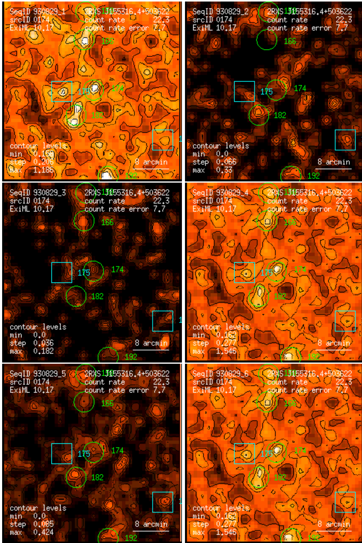
Figure 174: RASS 930829: detection 0174: band rate images, Gaussian filter: (1) PSPC channels 11 – 41, (2) 52 – 90, (3) 91 – 201, (4) 11 – 235, (5) 52 – 201, (6) 11 – 201. Broad band rates in counts/ks. Band rate contour levels in counts/ks/arcmin 2 .
